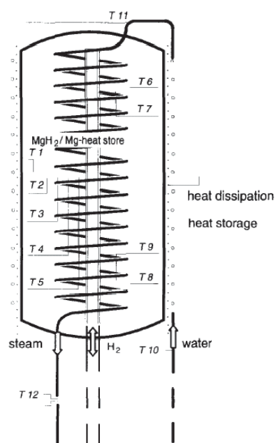
Figure 36. Left: layout of \text{MgH}_2 tank for a process steam generator. Right: The tank opened after 1.5 years of operation [345].
