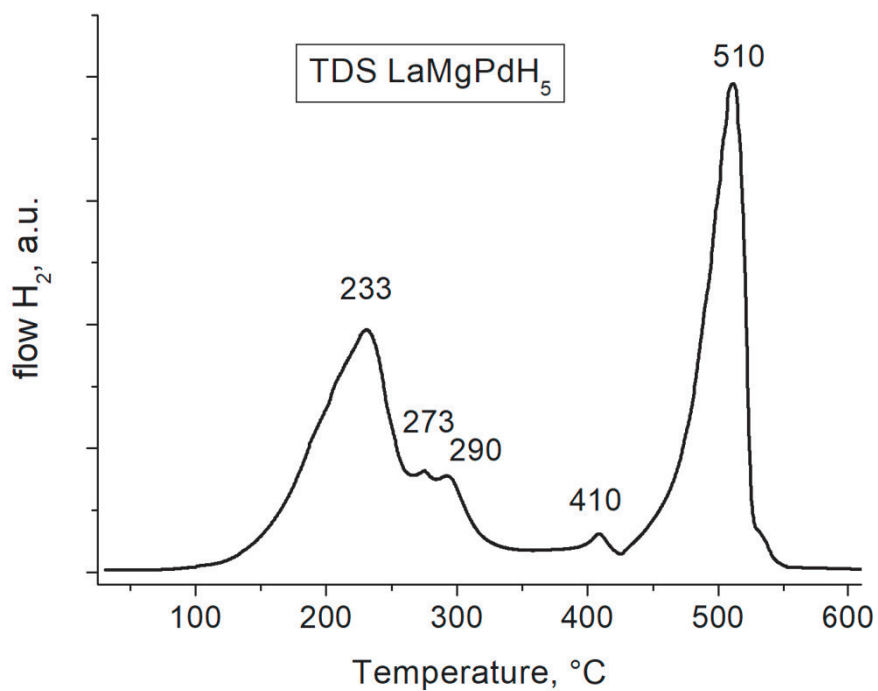
Figure 35. Vacuum Thermal Desorption Spectra of hydrogen from \text{LaMgPdH}_5 measured at a heating rate of 2^\circ\text{C}/\text{min}
