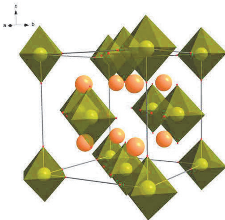
Figure 30. The crystal structure of \text{Mg}_2(\text{FeH}_6)_{0.5}(\text{CoH}_5)_{0.5} determined from Rietveld refinements of powder neutron and X-ray diffraction data. Mg yellow, Fe/Co green and H/D atoms - red dots in corners of the octahedra (D used for neutron diffraction).
