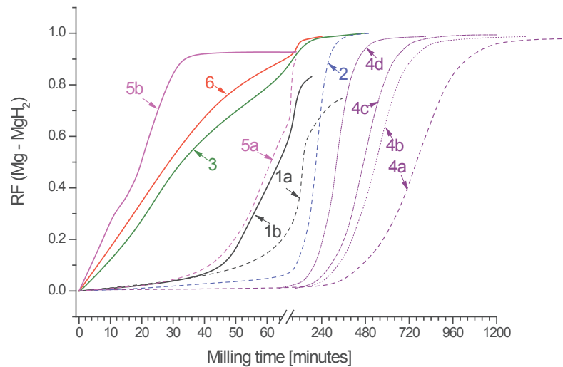
Figure 8. Hydrogenation of Mg during its ball milling in \text{H}_2
