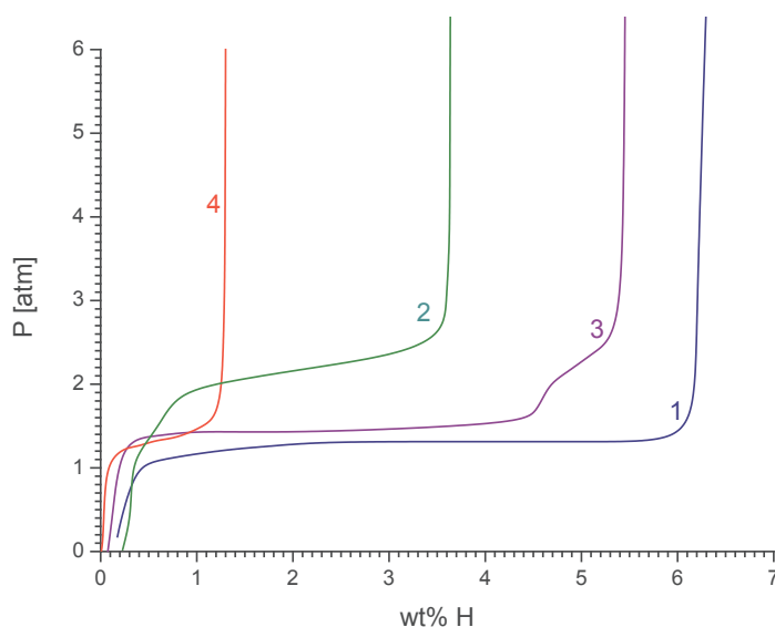
Figure 2. Pressure – composition isotherms ( \text{H}_2 desorption) for systems of \text{H}_2 gas with: 1 – Mg-based nanocomposite, T=300 °C [41]; 2 – \text{Mg}_2\text{Ni} , T=300 °C [41]; 3 – Mg – Ni – Mm eutectic alloy, T=300 °C [42]; 4 – \text{MmNi}_{4.9}\text{Sn}_{0.1} , T=22 °C [41]. Mm is lanthanum rich mischmetal.
