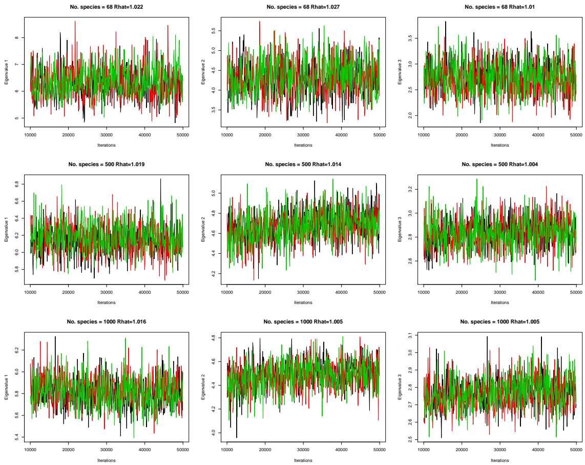
Figure S6: Traceplots for the posterior samples of the first three eigenvalues of \mathbf{S} . Each row corresponds to a different I and each column to a different eigenvalue. The \widehat{R} statistics are shown in the title of each figure.
