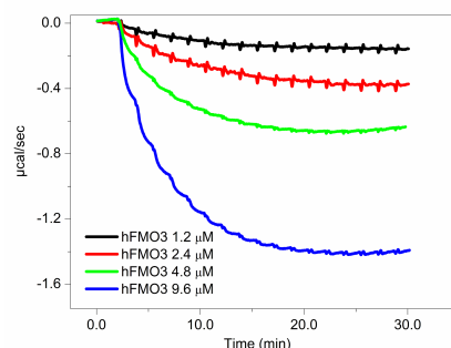
Fig.2 Multiple injections time-based ITC measurements of TMA ( 2 \mu\text{l} of 30 \mu\text{M} ) in 50 mM KPi buffer pH 7.4 containing hFMO3 ( 1.2 - 9.6 \mu\text{M} ) and 1.2 mM NADPH, 25^\circ\text{C} , 300 rpm stirring, mid-feedback mode, 120 seconds spacing between each injection.
