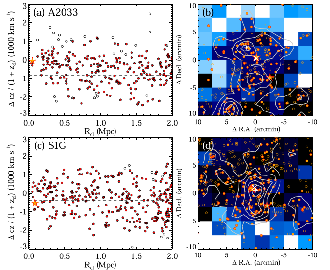
Figure 6. (a) R - v diagram centered on A2033. Open circles are the spectroscopic targets, and filled circles are the A2029 members within the caustics. The star symbol indicates the brightest galaxy of A2033. The horizontal dashed line indicates the mean redshift of A2029. (b) Galaxy distribution in the A2033 field. The background map is the two-dimensional redshift completeness map. Open and filled circles are the spectroscopic targets and A2033 members, respectively. The star symbol is the A2033 BGG. The gray contours are the number density map of the A2033 members. The cross is the X-ray peak from the Chandra observations (ObsID: 15167; PI: T.Reiprich). The plus symbol is the peak of the surface number density map of the A2033 members. (c) and (d) Same as (a) and (b) but for SIG. The cross in panel (d) is the X-ray peak determined based on the ROSAT data.
