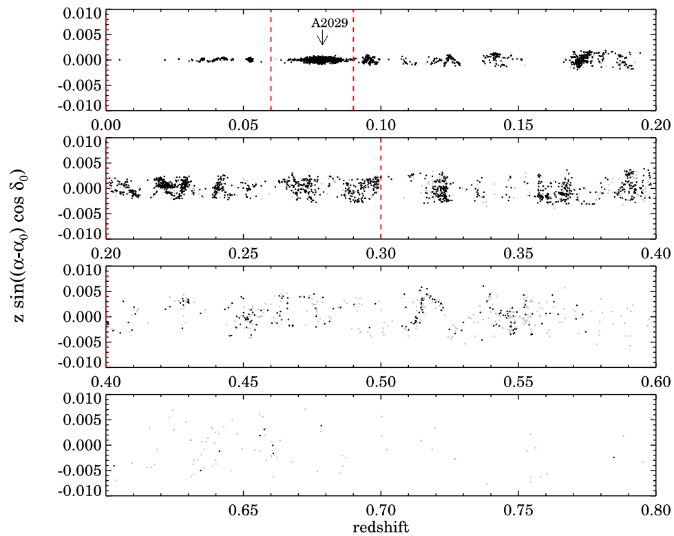
Figure 3. Cone diagram of the A2029 field within R_{cl} < 40' projected in the R.A. direction. Black (gray) points are the galaxies brighter (fainter) than r_{cModel,0} = 20.5 . Dashed vertical lines display the boundaries we use for identifying galaxy surface number densities that correspond to groups as described in Section 4.2.
