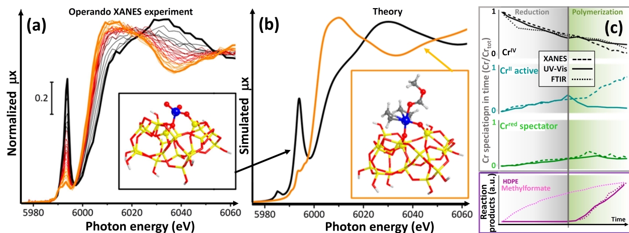
Fig. 3. Part (a): time evolution of the operando Cr K-edge XANES spectra of the Cr VI /SiO 2 catalyst (bold black) during reduction with ethylene (from black to bold red) and during ethylene polymerization at 150 °C (from bold red to bold orange). Spectra were collected in fluorescence mode (see Fig. 1a) at the BM23 beamline of the ESRF [232]. Part (b): simulated XANES spectra, computed with the FSMNES code [37, 38], of Cr VI /SiO 2 (black) and Cr II /SiO 2 in interaction with methylformate and ethylene (orange), and corresponding structural models used to compute the XANES spectra (insets), where silica support has a brutto formula of Si 21 O 48 H 10 . Part (c): time-resolved spectroscopic speciation along the three operando experiments: XANES (dashed curves), UV-vis-NIR (solid curves) and FTIR (dotted curves). Spectroscopic fingerprints of, from top to bottom: Cr VI (first component in the XANES PCA analysis; 21500 cm -1 UV-vis transition; and 1980 cm -1 FTIR band); Cr II in interaction with methylformate and ethylene (third second component in the PCA XANES analysis; and 9500 cm -1 UV-vis transition; spectator Cr species (third component in the PCA XANES analysis; and 15100 cm -1 UV-vis transition); HDPE (4400–4050 cm -1 UV-vis transition; and 2853 cm -1 FTIR band) and methylformate (1573 cm -1 FTIR band). Adapted with permission from Ref. [231], copyright American Chemical Society, (2017).
