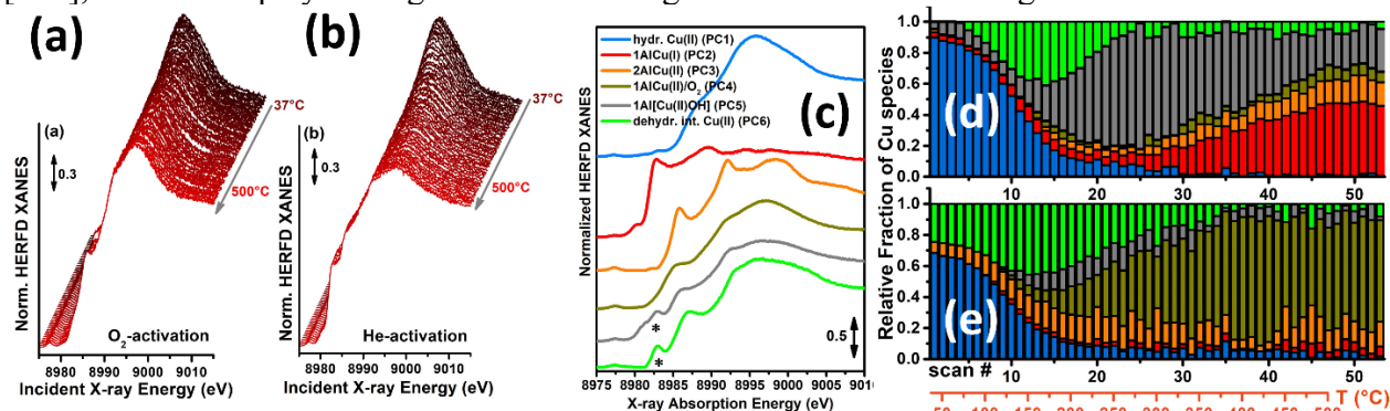
Fig. 8. Parts (a), (b): in situ temperature-dependent HERFD-XANES data collected during O 2 - and He-activations, respectively, for Cu-CHA (Si/Al = 12, Cu/Al = 0.5). Part (c): pure spectra isolated through MCR-ALS algorithm of the in situ HERFD-XANES datasets reported in parts (a) and (b). The * symbol indicates the presence of reconstruction artefacts in the form of spurious rising-edge peaks for spectra PC5 and PC6. The cause of these results can be identified in the presence of very minor contributions, whose Cu concentration profiles are completely embedded in the concentration window of much more abundant Cu species. (d), (e): concentration profiles for the pure HERFD-XANES spectra (reported in (c)) during He-activation (d) and O 2 -activation (e), plotted as a function of the scan number (2 min/scan) and of the related data collection temperature (orange axis, from 37 °C to 500 °C, plus ~ 15 min dwelling time in isothermal conditions at 500 °C). Bars have the same colors as the corresponding spectra in panel (c).
