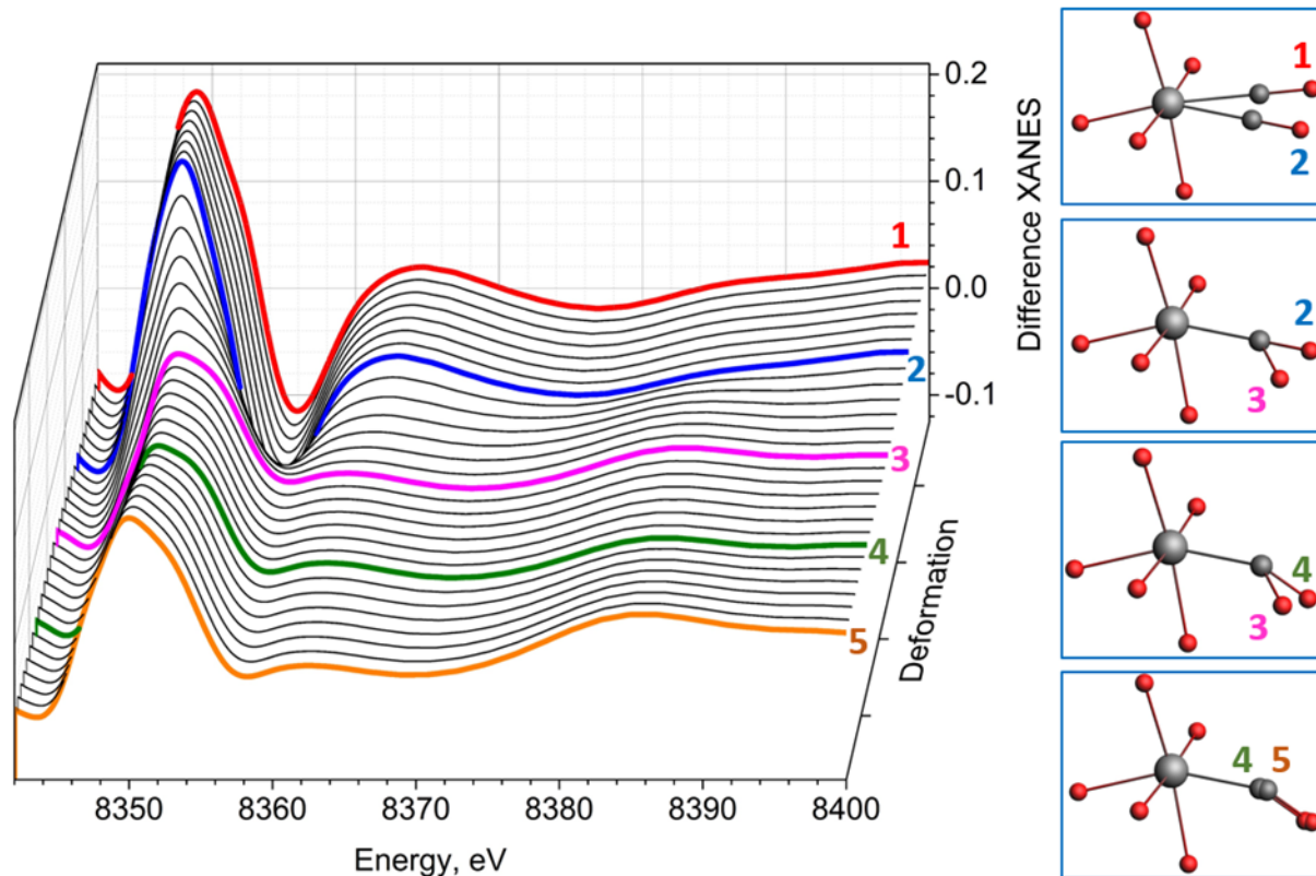
Fig. 11. Variation of the theoretical difference XANES spectra for the CPO-27-Ni/ CO adduct. The difference is calculated between spectra for the structure with adsorbed CO and that with naked \text{Ni}^{2+} (activated sample). The five bold colored curves correspond to the vertices of the trajectory in the 5-dimensional space [\text{R}_{\text{ads}}, \alpha_1, \alpha_2, \beta_1, \beta_2] , from 1 to 5 : [2.0, 0.0, 0.0, 0.0, 0.0]; [2.0, 20.0, 0.0, 0.0, 0.0]; [2.0, 20.0, 0.0, 45.0, 0.0]; [2.0, 20.0, 0.0, 45.0, 90.0]; [2.15, 20.0, 0.0, 45.0, 90.0], respectively.
