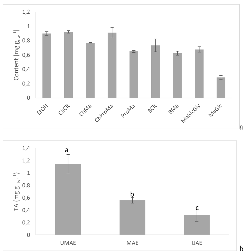
Figure 2. Total anthocyanins content (mg g -1 dw ) of prepared extract with different NADES (a) and extraction efficiency for grape pomace anthocyanins with ChCit under different irradiation (b). Total anthocyanins were expressed as a sum of identified anthocyanins. Content of anthocyanins were expressed as the means (n=3) \pm S.D. Presented value followed by different lower-case letters (a-c) are significantly different ( p < 0.05 ) as measured by Tukey's HSD test.
