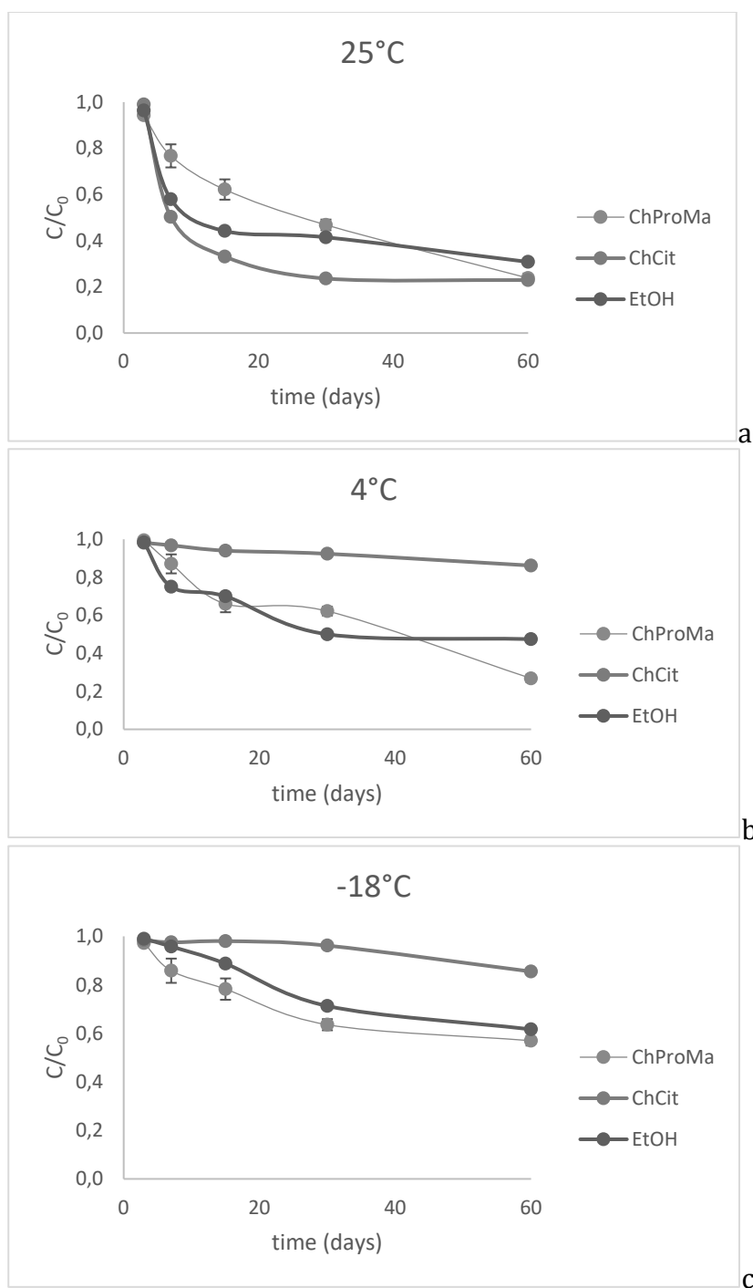
Figure 3. Degradation curve of anthocyanins in ChProMa- ChCit- and EtOH- extracts at 25°C (a), 4°C (b) and -18°C (c) through 60 days. Results were expressed as the means ( n=3 ) \pm S.D
