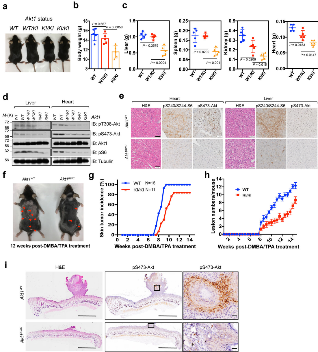
Fig. 2. Methylation deficient Akt1 knock-in mice display reduced body size/weight and resist to chemical carcinogen-induced skin tumorigenesis in vivo a , Mice derived from the same litter were imaged at age of 4 weeks old. b , The mice derived from the age of 4 weeks were weighed (including 15 male mice with 5 WT, 5 heterogeneous, and 5 homogeneous- Akt1 K140/142R genetic background status). Error bars are mean \pm s.e.m, n = 5 mice. P values were calculated using two-tailed unpaired Student's t test. c , The mice in ( b ) were euthanized and their organs were dissected and weighed. Error bars are mean \pm s.e.m, n = 5 mice. P values were calculated using two-tailed unpaired Student's t test. d , IB analysis of WCL derived from livers or hearts of WT (+/+), Akt1 K140/142R -knock-in heterogeneous (+/KI) or homogeneous (KI/KI) mice from the same litter at age of 4 weeks. The experiment was performed twice, independently, with similar results. e , Graphic representation of H&E and IHC staining of heart and liver tissues derived
