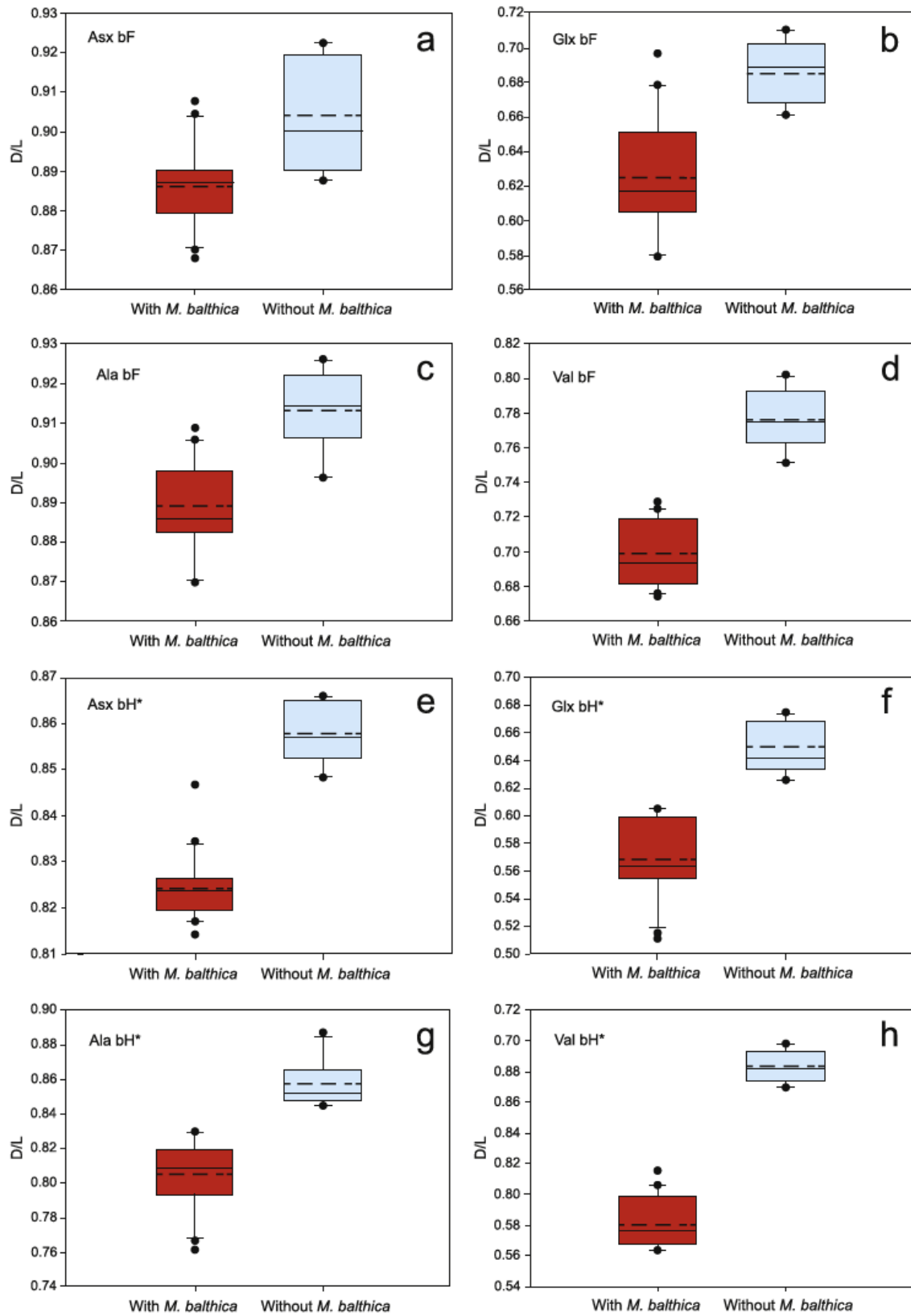
Fig. 17. Comparisons of amino acid data from the shells of Nucella lapillus from assemblages with (Sidstrand, Weybourne Hope, East Runton) and without (Bramerton, Covehithe) Macoma balthica . a-d. D/L values of Asx, Glx, Ala, Val for the free amino
