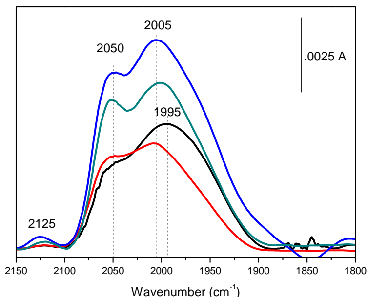
Figure 4. FTIR difference spectra collected upon the adsorption of 15 mbar CO at RT and subsequent outgassing at RT on monometallic Ru/ZrO 2 (black curve), and bimetallic AuRu/ZrO 2
