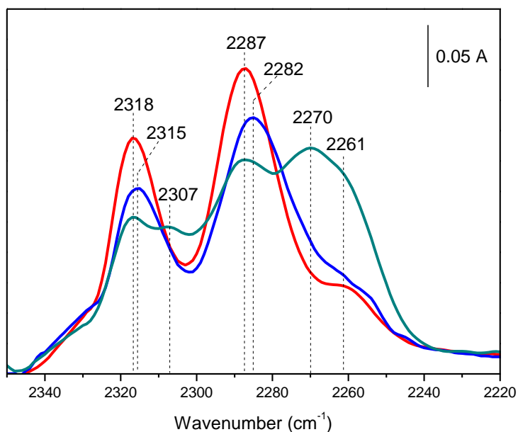
Figure 7. FTIR difference spectra collected upon the adsorption of 2 mbar CH 3 CN at RT on bimetallic AuRu/ZrO 2 (red curve), AuRu/Y-ZrO 2 (blue curve) and AuRu/La-ZrO 2 (cyan curve) catalysts. The spectra have been normalized on the weights of the pellets and on the specific surface areas of the supports.
