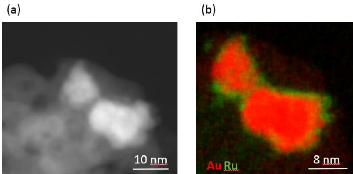
Figure SI-3. HAADF-STEM image of the AuRu/Y-ZrO 2 sample (section a) and quantified EDXS mapping (section b, Au,(red and Ru,green), showing the Ru NPs sitting on top of the Au NP.
