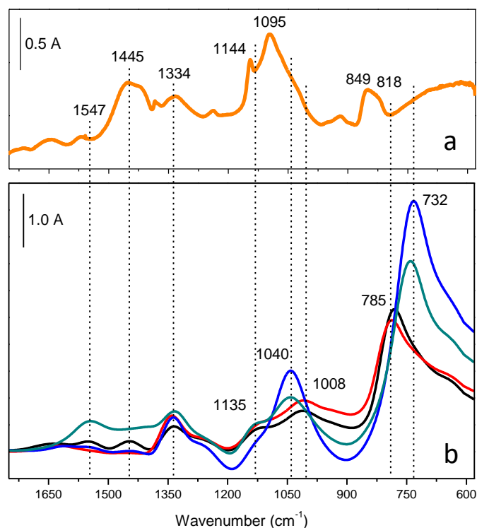
Figure 4. FTIR absorbance spectra of PVA in KBr (section a) and of monometallic Ru/ZrO 2 (black curve), bimetallic AuRu/ZrO 2 (red curve), AuRu/Y-ZrO 2 (blue curve) and AuRu/La-ZrO 2 (cyan curve) catalysts collected upon outgassing at 100 °C for 30 minutes (section b). The spectra in section b have been normalized on the weights of the pellets.
