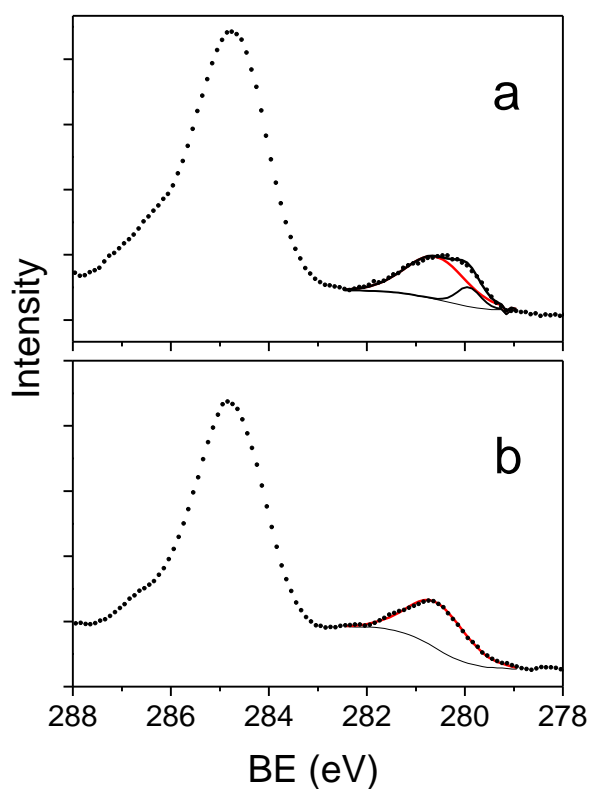
Figure 6. Ru 3d XP spectra (circles) for the samples Ru/ZrO 2 (a) and Au-Ru/ZrO 2 (b), along with the curve-fits. In both sections, the red line is the peak corresponding to the Ru x+ species, whereas in section (a) the peak of Ru 0 species is also reported as a black-line.
