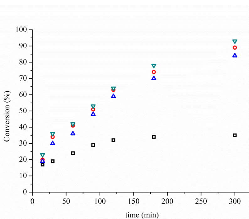
Figure 1. Reaction profile for monometallic Ru/ZrO 2 (black squares), and bimetallic AuRu/ZrO 2 (red circles), AuRu/Y-ZrO 2 (blue triangles) and AuRu/La-ZrO 2 (cyan triangles) catalysts.
