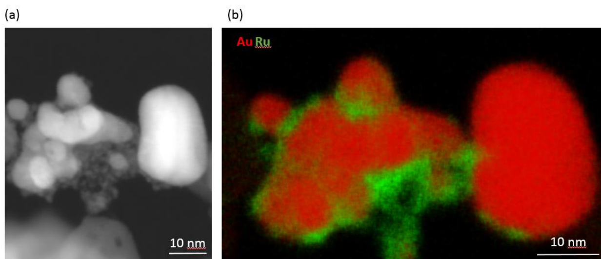
Figure SI-4. HAADF-STEM image of the AuRu/La-ZrO 2 sample (section a) and quantified EDXS mapping (section b, Au,(red and Ru,green), showing the Ru NPs sitting on top of the Au NP.
