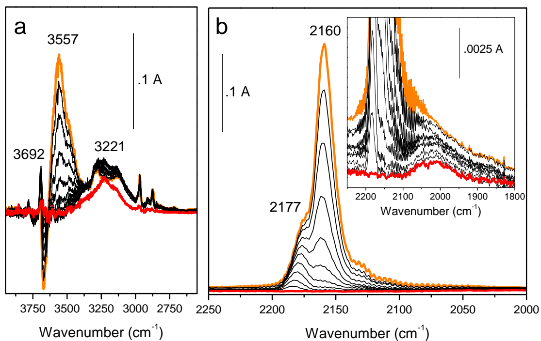
Figure SI-5. FTIR difference spectra collected on the Ru/ZrO 2 catalyst upon the inlet of 4 mbar CO at LNT (orange curve) and at decreasing CO pressures (black curves up to the red one) in the OH stretching region (section a) and in the carbonylic region (section b). Inset: zoom on the component at 2000-2050 cm -1 .
