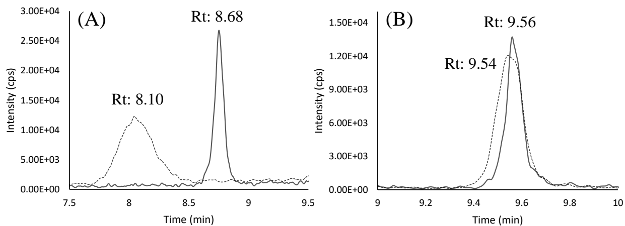
Figure 1 – MRM chromatograms of (A) PFPeA and (B) PFBuS reference standard solutions (concentration 500 ng/L) prepared in the QuEChERS procedural blank as such (dashed line) and acidified with 0.1% ( v/v ) formic acid (solid line).
