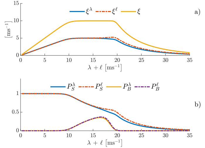
Fig. 14. Flows with different priorities: a) system throughput, b) P_S and P_B
