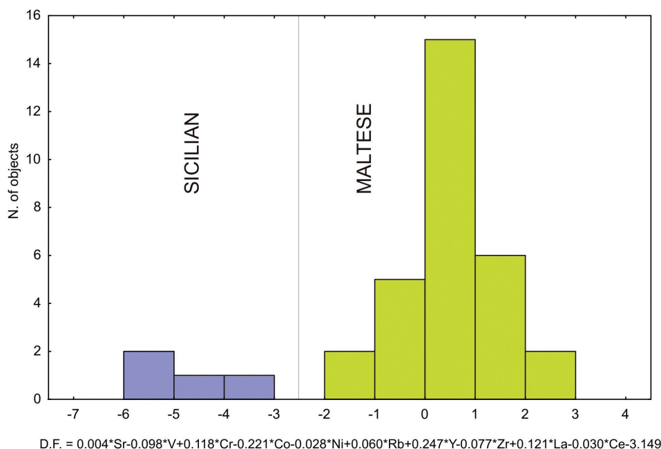
Figure 8. Discriminant analysis result expressed as histogram of the values of discriminant function (D.F.) for each samples. The diagram shows the bimodal distribution due to the individuation of two groups (i.e. Maltese and Sicilian pottery).
