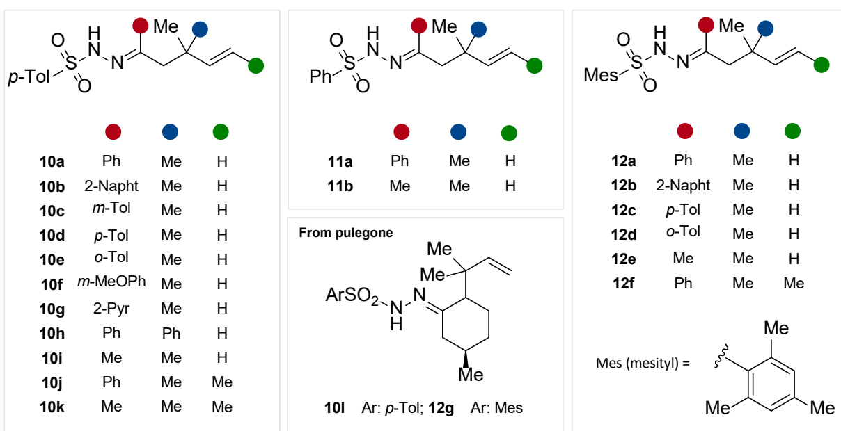
Scheme 3 Synthesis and list of the \beta -hindered \gamma,\delta -unsaturated hydrazones
