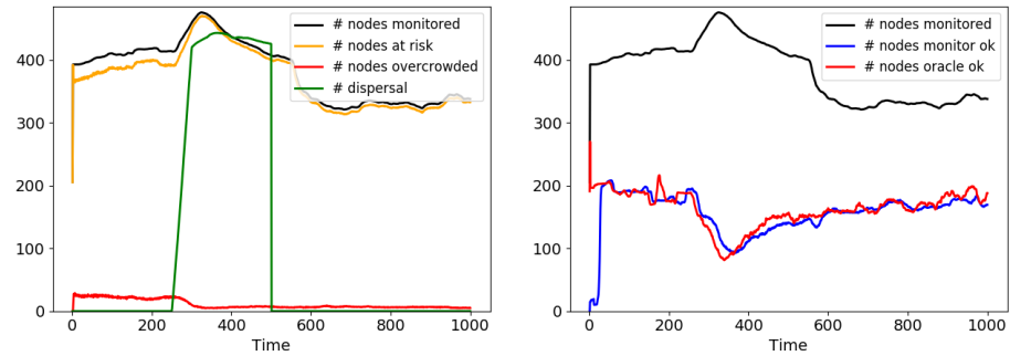
(a) Number of devices that perceive a dangerous (red line) or moderate (orange line) overcrowding, monitored (black line), and following dispersal advices (green line). (b) Number of monitored devices (black line) that satisfy the property according to the oracle (red line) and the monitor (blue line).
