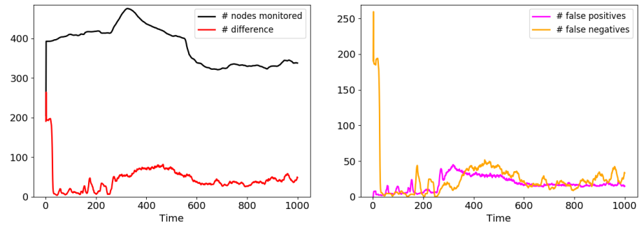
(c) Number of monitored devices (black line) for which the oracle and the monitor provide a different response (red line). (d) Detail of the error in terms of the number of devices providing false positives (magenta line) and false negatives (orange line).
