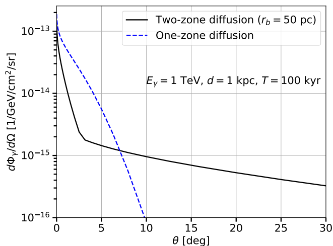
FIG. 3: Surface brightness for the ICS flux as a function of the angle from the central pulsar, setting d = 1 kpc, T = 100 kyr, D_0 = 2 \cdot 10^{26} , E_\gamma = 1 TeV and assuming the one or two-zone diffusion models ( r_b = 50 pc, equivalent to an angular distance of \theta = 2.86^\circ ).
