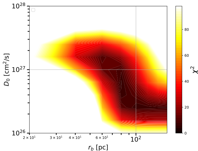
FIG. 11: Results of the fit to the HESS J1825-137 PWN surface brightness varying D_0 and r_b . The color bar describes the value of \chi^2 .
