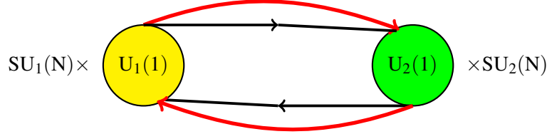
Figure 2: The quiver diagram associated with the \mathbb{C}^2/\mathbb{Z}_2 Kleinian singularity, whose resolution is the Eguchi Hanson HyperKähler manifold. In the two nodes, which correspond to the two irreducible one-dimensional representations of \mathbb{Z}_2 we place the two gauge groups SU_{1,2}(N) \times U_{1,2}(1) . The scalar multiplets correspond to the two directed lines going from one to the other node and are in the bi-fundamental representation of the mentioned node groups. The HyperKähler quotient is done with respect to the relative U(1) group, the overall U(1) being the irrelevant barycentric group.
