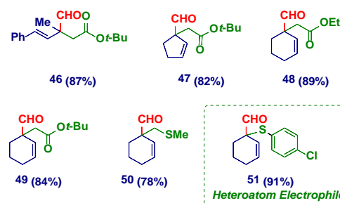
Scheme 3. Synthesis of fully substituted quaternary \alpha -methyl aldehydes.
