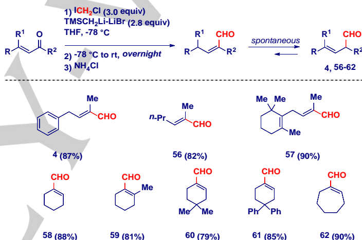
Scheme 6. Synthesis of \alpha,\beta -unsaturated aldehydes through homologation-isomerization followed by acidic quenching.
