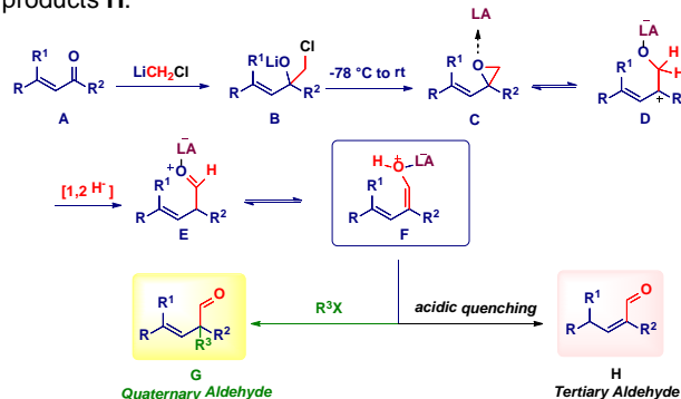
Scheme 4. Plausible mechanism.
