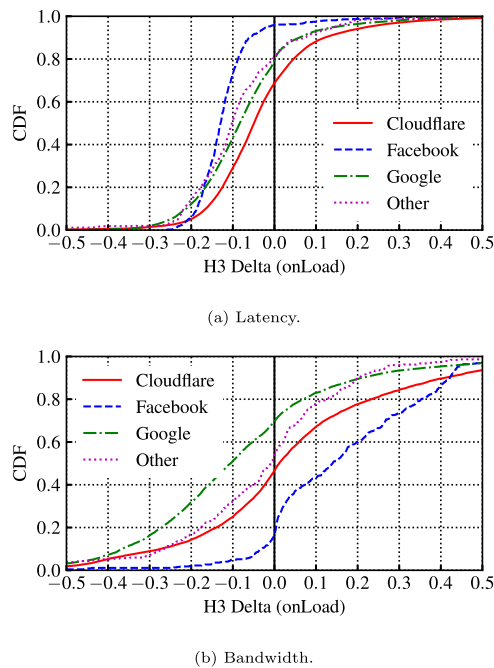
Fig. 8. onLoad H3 Delta by website provider for scenarios with extra-latency and bandwidth limit ( BrowserTime-Web dataset). (For interpretation of the references to color in this figure legend, the reader is referred to the web version of this article.)
