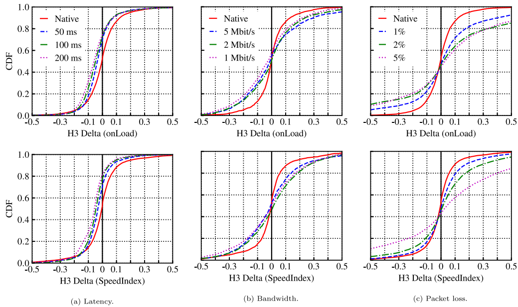
Fig. 7. H3 Delta on different scenarios. onLoad (top) and SpeedIndex (bottom). Negative values indicate that HTTP/3 is faster ( BrowserTime-Web dataset).
