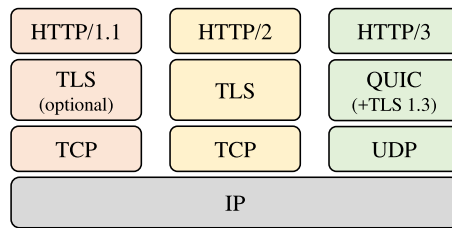
Fig. 1. Protocol stack for different HTTP versions.
