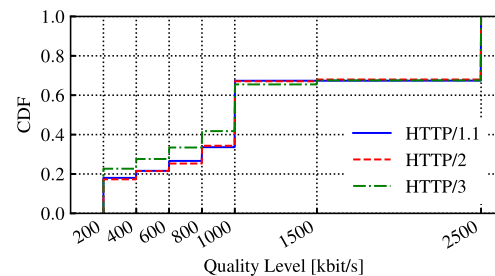
Fig. 13. Distribution of chunks resolution with limited bandwidth ( BrowserTime-Video dataset).
