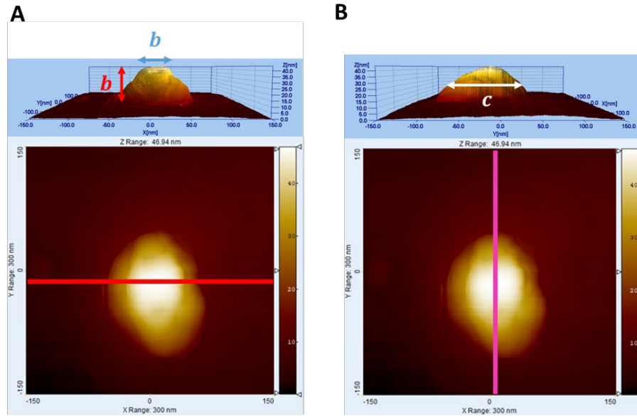
Figure 4. 2D and 3D topographies of a nanobipyramid by mAFM. Determination of (A) ' b ' and (B) ' c ' sizes.
