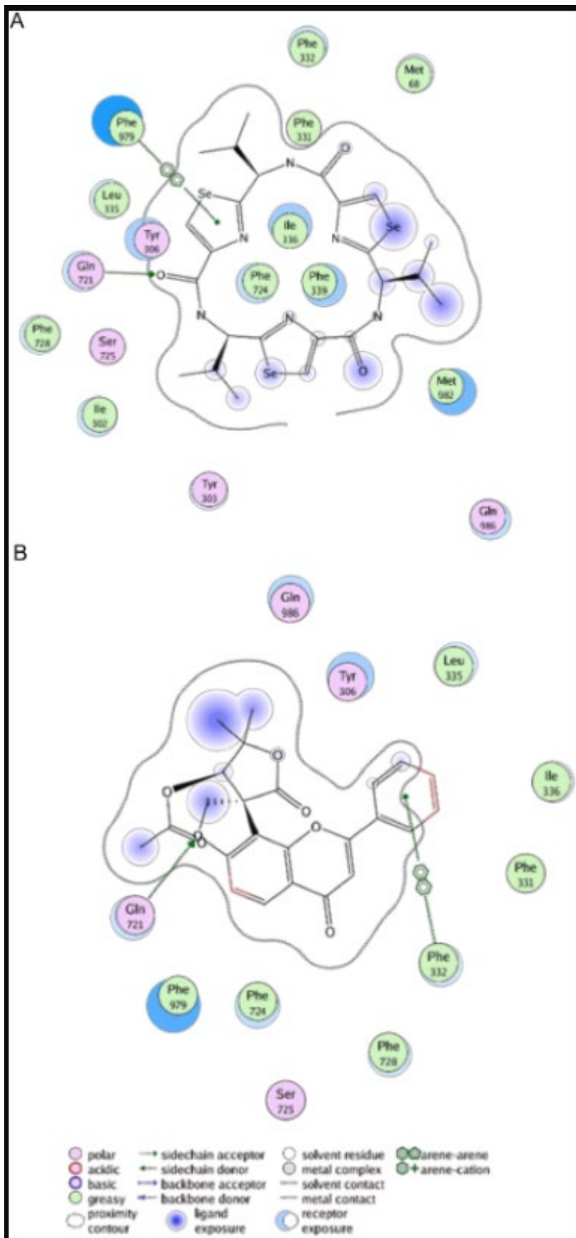
Fig.8 Modeling of the interactions between QZ59-RRR or Glabratephrin and Pgp. A-B. The functional groups involved in the interaction between QZ59-RRR (panel A) or Glabratephrin (panel B) and Pgp (4M2S) were displayed.
