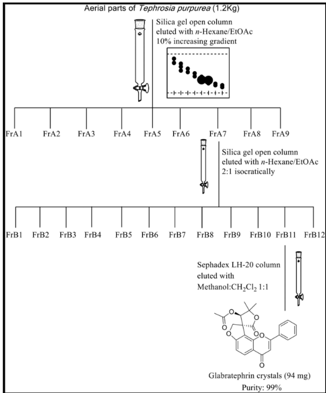
Fig.1 Extraction procedure and structure of Glabratephrin.
