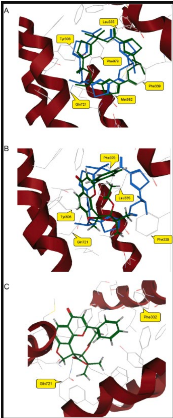
Fig.7 Docking of QZ59-RRR or Glabratephrin on Pgp. A. Superposition of the co-crystallized ligand QZ59-RRR (blue) and re-docked ligand QZ59-RRR (green) on Pgp (4M2S). B. Superposition of the co-crystallized ligand QZ59-RRR (blue) and Glabratephrin (green) on Pgp (4M2S). C. Putative binding mode of Glab with on Pgp (4M2S).
