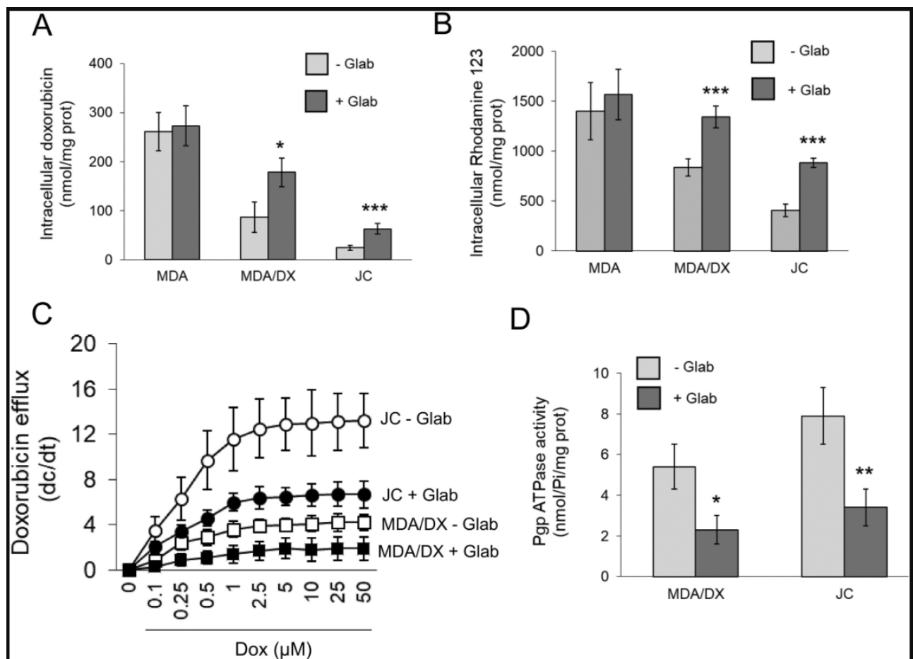
Fig.6 Glabratephrin reduces Pgp activity. A. MDA-MB-231 cells (MDA), MDA-MB-231/DX cells (MDA/DX) and JC cells were incubated 24 h with 5 \mu M doxorubicin (Dox), in the absence (-) or presence (+) of 100 nM Glabratephrin (Glab). The intracellular drug accumulation was measured fluorimetrically in duplicates. Data are presented as means \pm SD (n = 3). Glab-treated vs. untreated cells: * p < 0.05; *** p < 0.001. B. Cells were incubated 20 min with 1 \mu g/ml Rhodamine 123, in the absence (-) or presence (+) of 100 nM Glab. The intracellular accumulation of Rhodamine 123 was measured fluorimetrically in duplicates. Data are presented as means \pm SD (n = 3). Glab-treated vs. untreated cells: *** p < 0.001. C. Cells were incubated 10 min with increasing concentrations of Dox (0.5–50 \mu M), in the absence (-) or presence (+) of 100 nM Glab. One series of dishes was analyzed for the intracellular Dox concentration (c1); a second series was washed and let in the incubator for additional 10 min, then analyzed for the intracellular Dox concentration (c2) as well. The dc/dt value was considered indicative of Dox velocity of efflux. Data are presented as means \pm SD (n = 3). D. Cells were grown 24 h in the absence (-) or presence (+) of 100 nM Glab. The Pgp ATPase activity was measured spectrophotometrically in duplicates. Data are presented as means \pm SD (n = 3). Glab-treated vs. untreated cells: * p < 0.05; ** p < 0.01.
