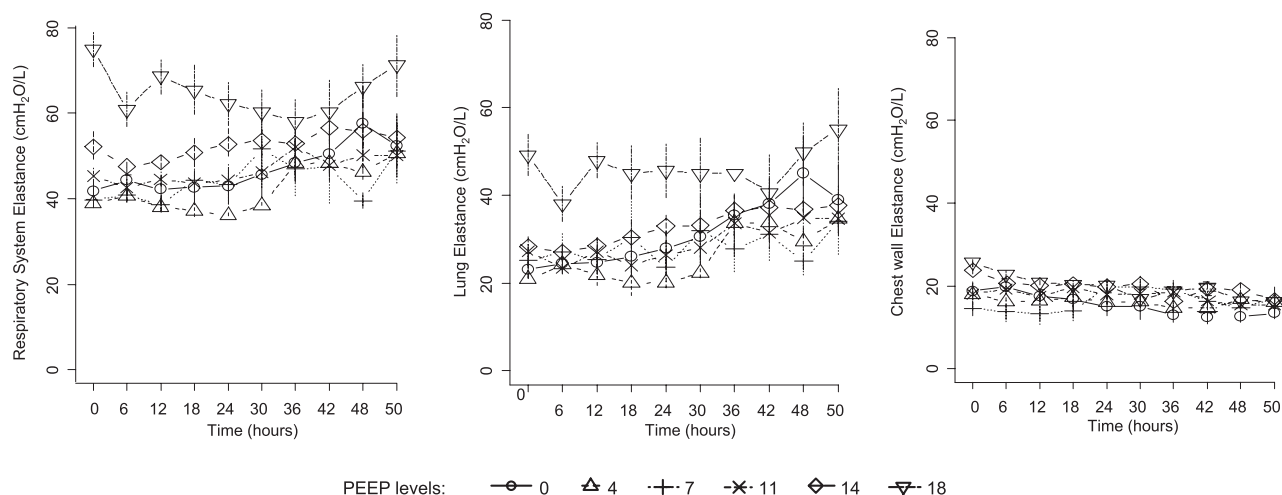
Fig. 2. Time course of respiratory system elastance (linear mixed effects model: time, P < 0.001 ; positive end-expiratory pressure [PEEP], P < 0.001 ; PEEP:time interaction, P = 0.445 ; left ), lung elastance (linear mixed effects model: time, P < 0.001 ; PEEP, P = 0.002 ; PEEP:time interaction, P = 0.499 ; middle ), and chest wall elastance (linear mixed effects model: time, P = 0.005 ; PEEP, P = 0.103 ; PEEP:time interaction, P = 0.125 ; right ) in the different PEEP groups.
