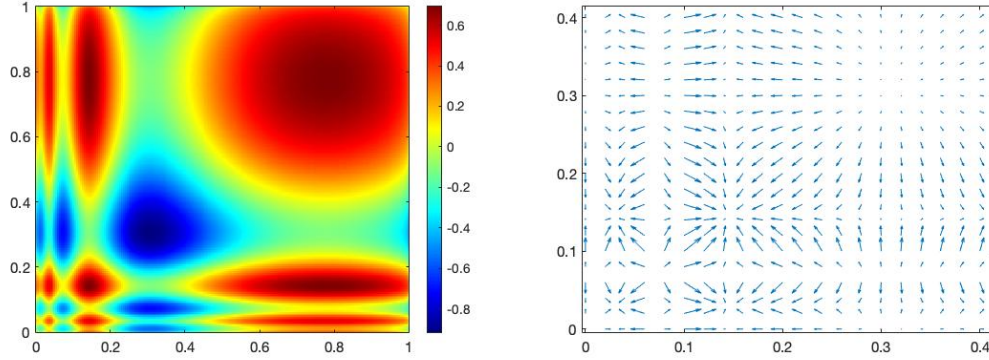
FIG 1. An example of a spatially heterogeneous potential B (left) and the corresponding gradient vector field \nabla B (right). Note the axis scales are different for clarity.
