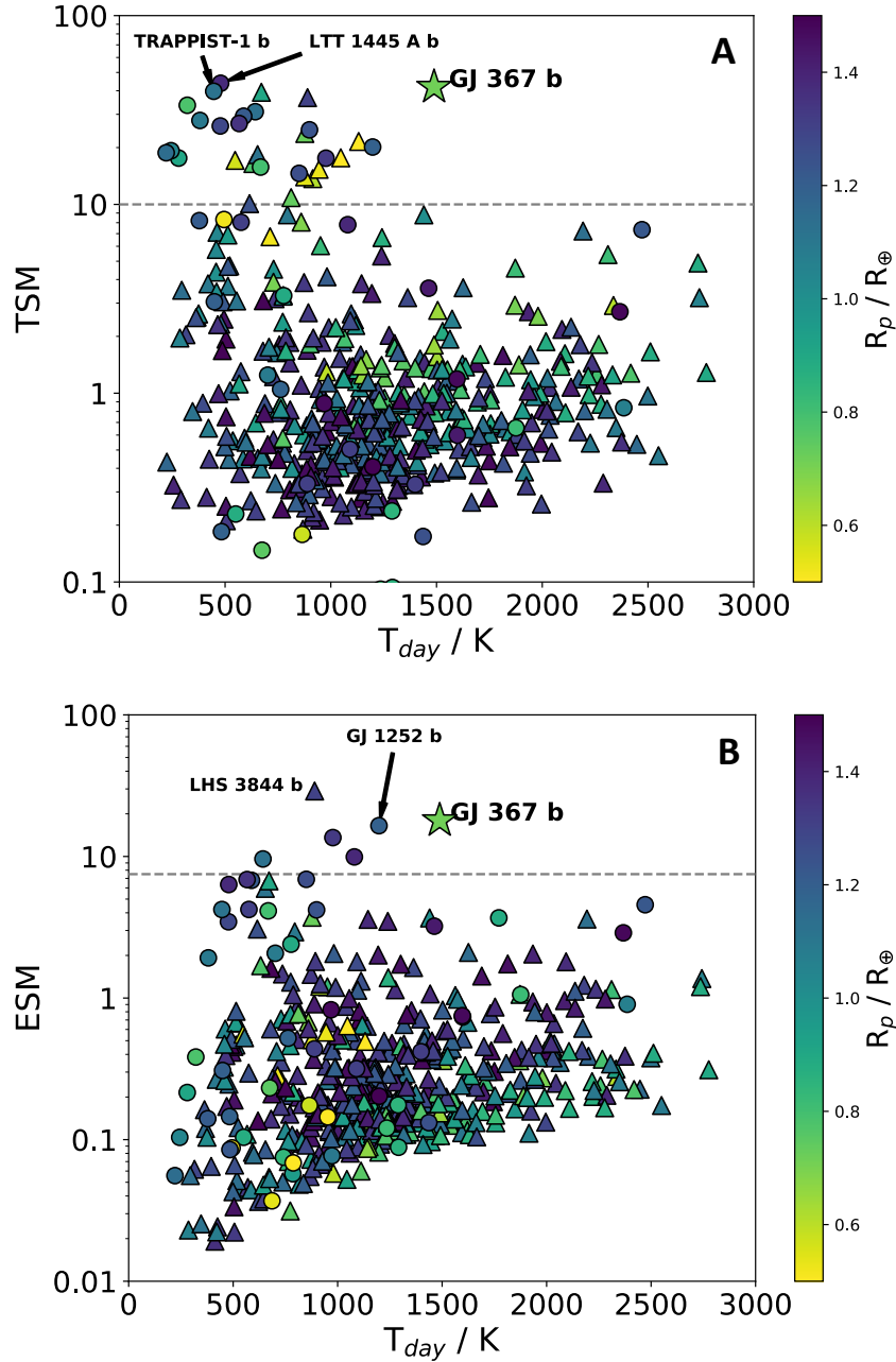
Fig. S10. Transmission and thermal emission metrics of known terrestrial planets with R_p < 1.5 R_\oplus . (A) Transmission metric, TSM. (B) Thermal emission metric, ESM. In both panels, planets directly measured masses are denoted by circles. Triangles denote planets with masses estimates from an empirical mass-radius relation (124). The TSM and ESM of GJ 367b are indicated by the star symbol. The color of each point indicates the size of the planet relative to Earth. The threshold TSM and ESM values are denoted by the grey lines. Because GJ 367b lies above these lines, it is suitable atmospheric studies. Selected other planets are labelled.
