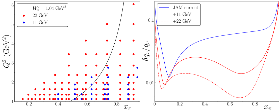
Figure 15: (Left) The kinematics of the 11 GeV (blue) and 22 GeV (red) points in Q^2 versus x_\pi along with the line of W_\pi^2 = 1.04 GeV ^2 . Multiple bins in t are on each red point. (Right) The impact on the valence quark distribution from the JLab TDIS experiments.
