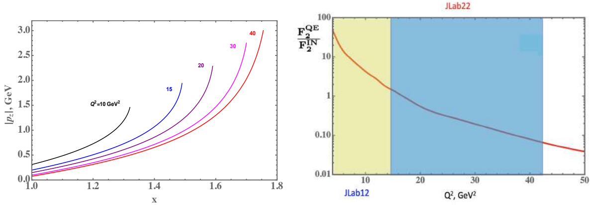
Figure 51: Left: Absolute value of internal longitudinal momenta for DIS from bound nucleon with produced final mass of W = 2 GeV at different Q^2 . Right: Ratio of quasielastic to DIS contribution of the nuclear structure function F_2 for x = 1.5 and different Q^2 . No EMC effects are taken into account in this estimation.
