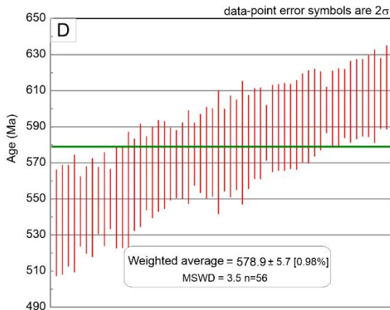
Figure 32 - Andrelândia Nappe (sample NESG-401): a) BSE images, X-ray maps (Y and Th) of monazites showing structural position, textural relationships, and internal zoning; b) Y_2O_3 (wt%) vs. age plot; c) ThO_2 (wt%) vs. age plot; d) weighted average diagram for monazite core dates; e) weighted average diagram for monazite enclosed in Ky.
