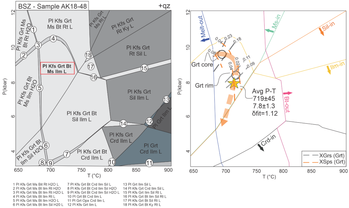
Figure 16 - P-T isochemical phase diagram in the MnNCKFMASHT system for AK18-48 (BSZ hanging-wall). The left diagram highlights the quadri-variant field for peak assemblage Qz+Pl+Kfs+Grt+Ms+Bt+Ilm+L . The right diagram shows the main minerals stability curves and P-T path based on mineral isopleths and THERMOCALC average P-T.
