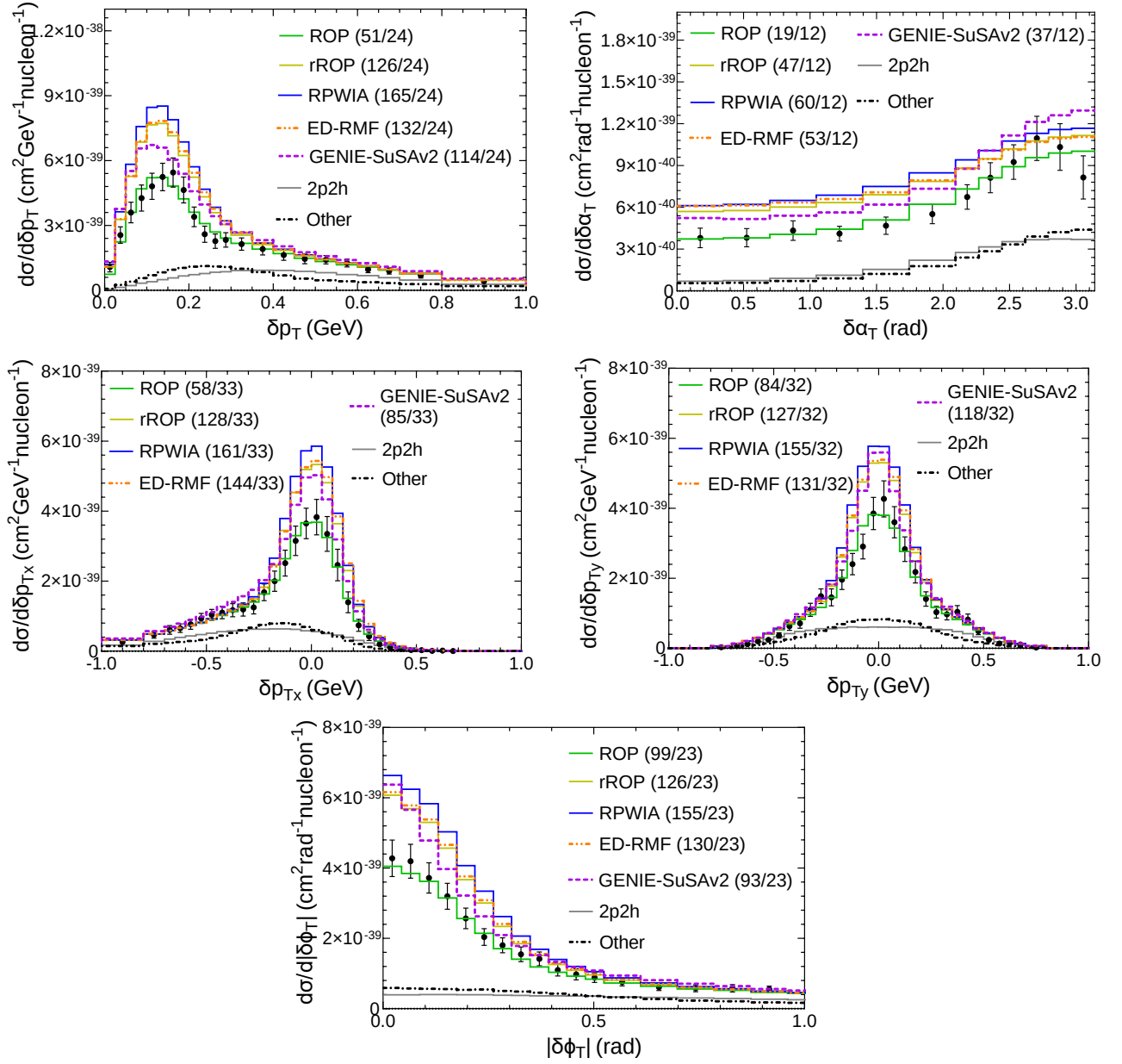
Figure 5.10: MINERνA 1\mu\text{CC}0\pi\text{Np} semi-inclusive \nu_\mu-^{12}\text{C} cross sections as function of the transverse kinematic imbalances \delta p_T , \delta p_{Tx} , \delta p_{Ty} , \delta\alpha_T and |\delta\phi_T| . All curves include the 2p2h and pion absorption (denoted “other”) contributions evaluated using GENIE (shown separately). The original paper from MINERνA was [117] but the cross-section measurements shown here were taken from [116] which corrected a mismodeling in GENIE’s elastic FSI that affected the cross-section measurements presented in the first paper. Notice that the convention used in [116] to define the x and y axis to project \delta p_T on is the opposite to the convention used in this thesis. The \chi^2/d.o.f. ratio is given in brackets in the legend of each distribution.
