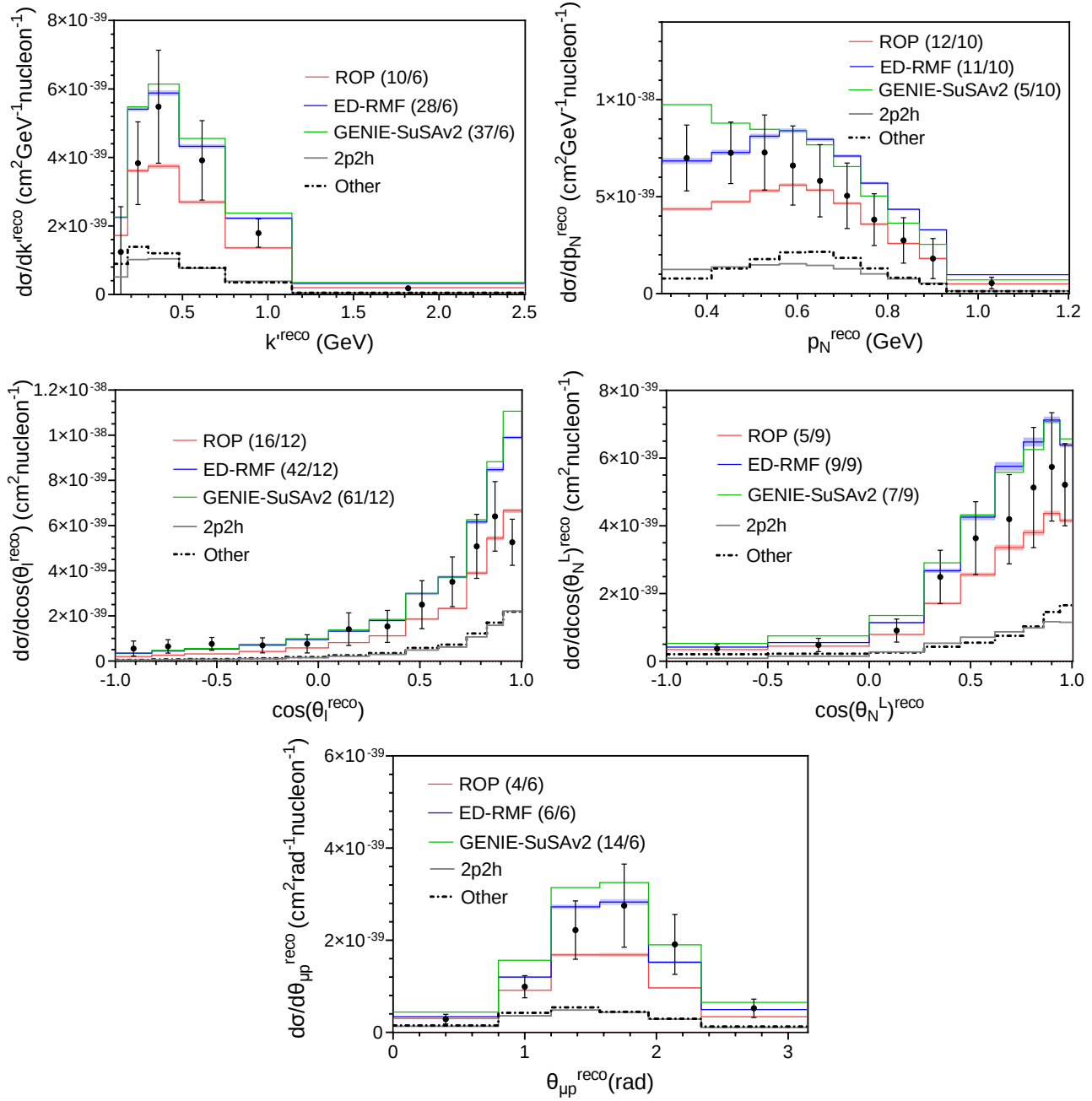
Figure 5-11: MicroBooNE 1\mu\text{CC}0\pi\text{Np} semi-inclusive \nu_\mu-^{40}\text{Ar} cross sections as function of the reconstructed muon and proton momenta and scattering angles and the opening angle \theta_{\mu p}^{\text{reco}} . All curves include the 2p2h and pion absorption (denoted “other”) contributions evaluated using GENIE (shown separately). Experimental results are from [118]. The bands, drawn for the ED-RMF and ROP models, represent the uncertainties associated with the modeling of the initial nuclear state. The \chi^2/\text{d.o.f.} ratio is given in brackets in the legend of each distribution.
