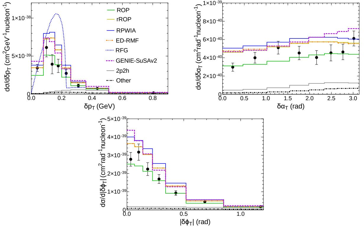
Figure 5.8: T2K 1\mu\text{CC}0\pi\text{Np} semi-inclusive \nu_\mu-^{12}\text{C} cross sections as function of the transverse kinematic imbalances \delta p_T , \delta\alpha_T and |\delta\phi_T| . All curves include the 2p2h and pion absorption (denoted “other”) contributions evaluated using GENIE (shown separately). Cross-section measurements taken from [115].
