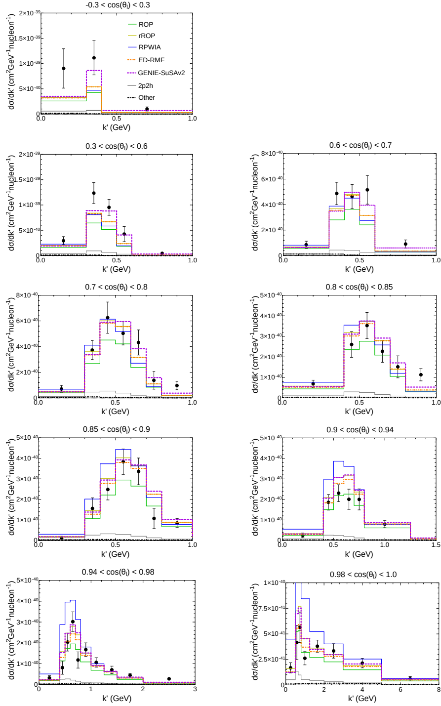
Figure 5.1: T2K 1\mu\text{CC}0\pi0p semi-inclusive \nu_\mu - ^{12}\text{C} cross section without protons in the final state with momenta above 0.5 GeV as function of the muon kinematics. All curves include the 2p2h and pion absorption (denoted “other”) contributions evaluated using GENIE (shown separately). Cross-section measurements taken from [115].
