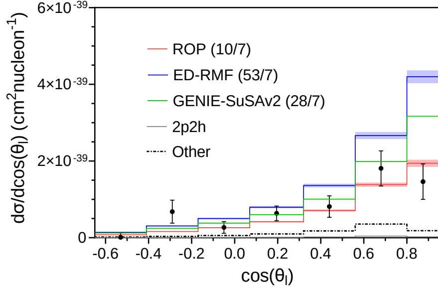
Figure 5.14: MicroBooNE 1\mu\text{CC}0\pi1p semi-inclusive \nu_\mu-^{40}\text{Ar} cross sections as function of the muon scattering angle. All curves include the 2p2h and pion absorption (denoted “other”) contributions evaluated using GENIE (shown separately). Experimental results were taken from [119]. The bands drawn for the ED-RMF and ROP models are related with the uncertainties associated with the modeling of the initial nuclear state. The \chi^2/d.o.f. ratio is given in brackets in the legend of each distribution.
