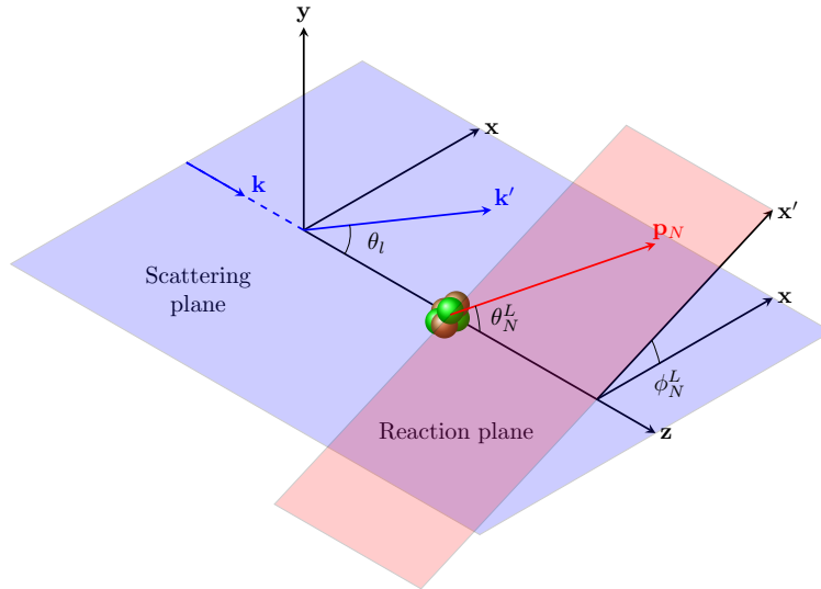
Figure 2.3: Definition of the coordinate system where the direction of the incoming neutrino k is fixed along the z -axis. The leptons are contained in the denominated scattering plane, while the ejected nucleon with momentum p_N and polar angle with respect to the neutrino direction \theta_N^L is contained in the so-called reaction plane, which forms an angle \phi_N^L with the scattering plane.
