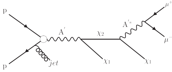
FIG. 1. Feynman diagram of IDM production and decay in pp collisions. The heavier state \chi_2 can be long-lived and decays to \chi_1 and to a muon pair via an off-shell dark photon A' .
