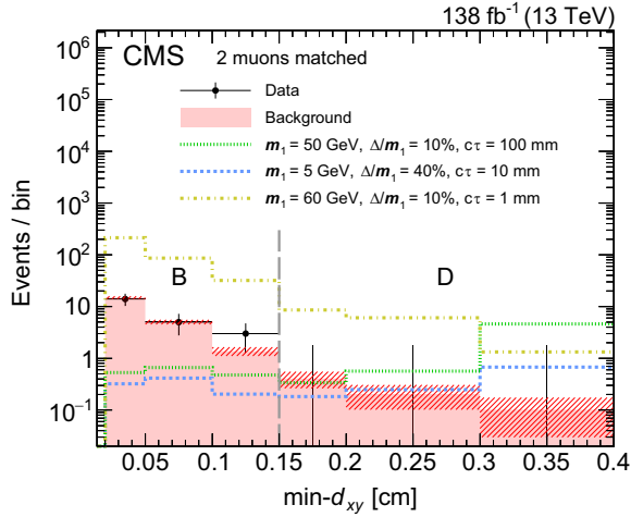
FIG. 3. Measured \min-d_{xy} distribution in the two-match category, after requiring the \min-d_{xy} muon to pass the isolation requirement J_{\text{PF}}^{\text{rel}} < 0.25 (i.e., the B and D bins of the ABCD plane). Overlaid with a red histogram is the background predicted from the region of the ABCD plane failing the same requirement (the A and C bins), as well as three signal benchmark hypotheses (as defined in the legends), assuming \alpha_D is equal to the electromagnetic (EM) fine-structure constant \alpha_{\text{EM}} . The red hatched bands correspond to the background prediction uncertainty. The last bin includes the overflow.
