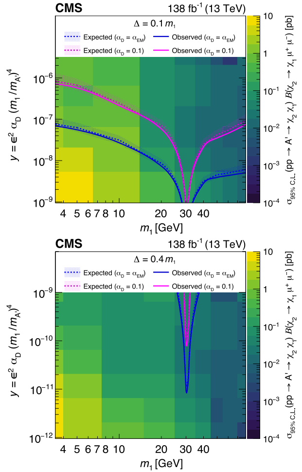
FIG. 4. Two-dimensional exclusion surfaces for \Delta = 0.1 m_1 (top) and 0.4 m_1 (bottom), as functions of the DM mass m_1 and the signal strength y , with m_{A'} = 3m_1 . Filled histograms denote observed limits on \sigma(pp \rightarrow A' \rightarrow \chi_2 \chi_1) \mathcal{B}(\chi_2 \rightarrow \chi_1 \mu^+ \mu^-) . Solid (dashed) curves denote the observed (expected) exclusion limits at 95% C.L., with 68% C.L. uncertainty bands around the expectation. Regions above the curves are excluded, depending on the \alpha_D hypothesis: \alpha_D = \alpha_{\text{EM}} (dark blue) or 0.1 (light magenta). The sensitivity is higher in the region near m_1 \approx 30 GeV or m_{A'} \approx 90 GeV because of the A' mixing with the Z boson in that mass range.
