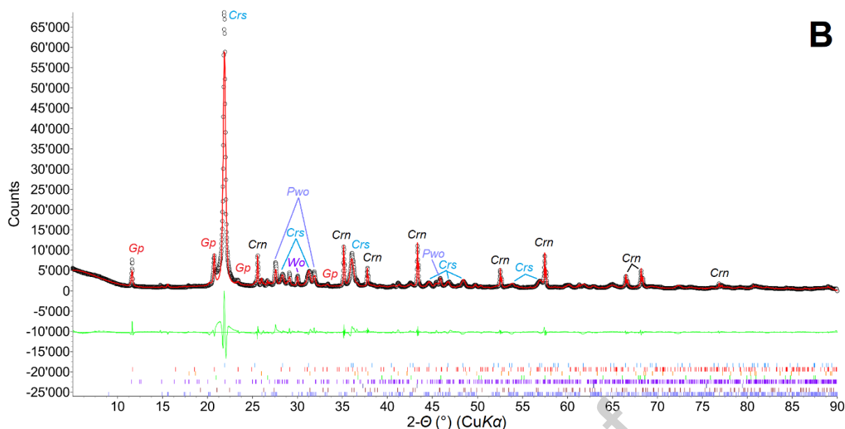
Figure 4 – Rietveld refinement plots of the XRPD patterns collected at RT for the samples investigated (A and B represent Rietveld plots for samples A1 and A2, respectively). The experimental profile is represented by black dots, the continuous red line is the calculated pattern, while the lower green curve is the difference between calculated and observed intensities. Vertical ticks mark the position of the reflections for the identified phases. Peaks belonging to the major constituents are also highlighted along with that of corundum (used as an internal standard). Namely, Crn, Crs, Gp, Pwo, Tlc, and Wo stand for corundum, cristobalite, gypsum, pseudowollastonite, talc, and wollastonite, respectively (Warr, 2021).
