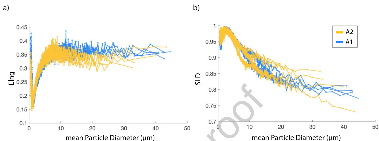
Figure 2 – Morphological variability of the grains from the two alginate samples (A1, A2). Moving average elongation, EIng , (a) and solidity, SLD , (b) are used to monitor the shape versus size variability of the grains.
