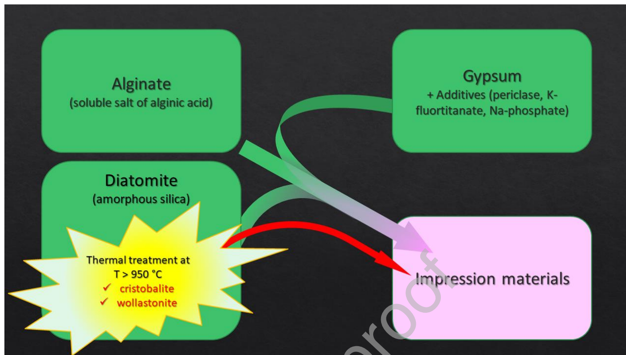
Figure 7 – Schematic representation of the preparation of impression alginate materials: alginate salts are mixed with diatomite and gypsum. In diatomite, amorphous silica has been partially converted to cristobalite by high temperature treatment. In the same process, wollastonite is obtained by reaction of silica and calcium carbonate.
