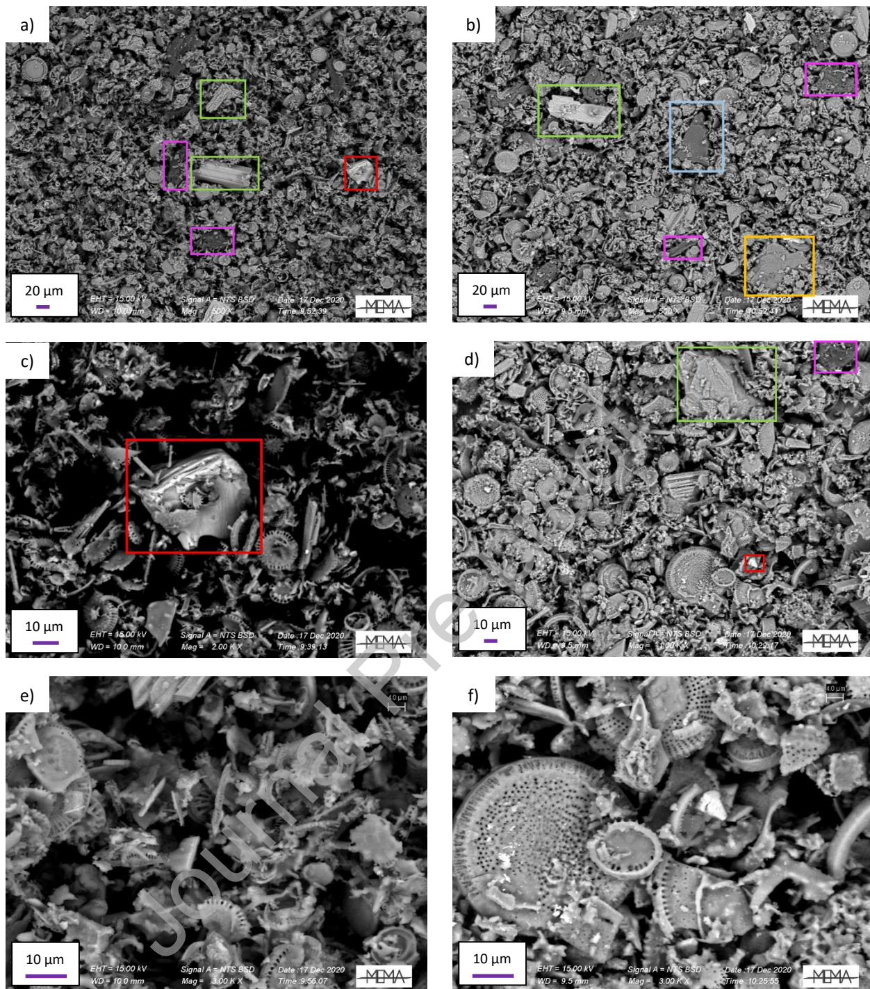
Figure 3 – Backscattered electron micrographs of the two samples investigated. a, c and e sample A1, b, d and f sample A2. Green, cyan, pink, yellow and red rectangles highlight particles of Ca sulfate, periclase, Na alginate, talc and K fluortitanate, respectively. Most of the unhighlighted particles consist of amorphous (or crystalline) silica (especially those with the typical diatomite shells). Magnification: 500X (a and b), 1000X (d), 2000X (c), 3000X (e and f).
