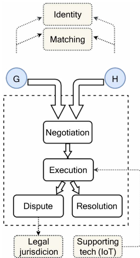
Figure 1. dAirBnB: decentralized accommodation rentals. Gaia (G) and Herbert (H) have undergone some form of digital identification, and their offer and demand matched. They have negotiated the terms of a rental contract in the form of a protocol that will be executed as a smart contract. Disputes may be escalated to a judiciary system (outside of the smart contract, which is represented by the dashed square). Supporting technology interacts with the contract.
