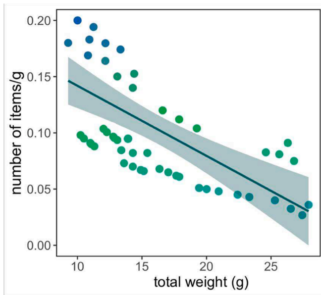
Fig. 5. Relationship between total weight (g) of Procambarus clarkii and number of microplastic items/g in the digestive tract.
