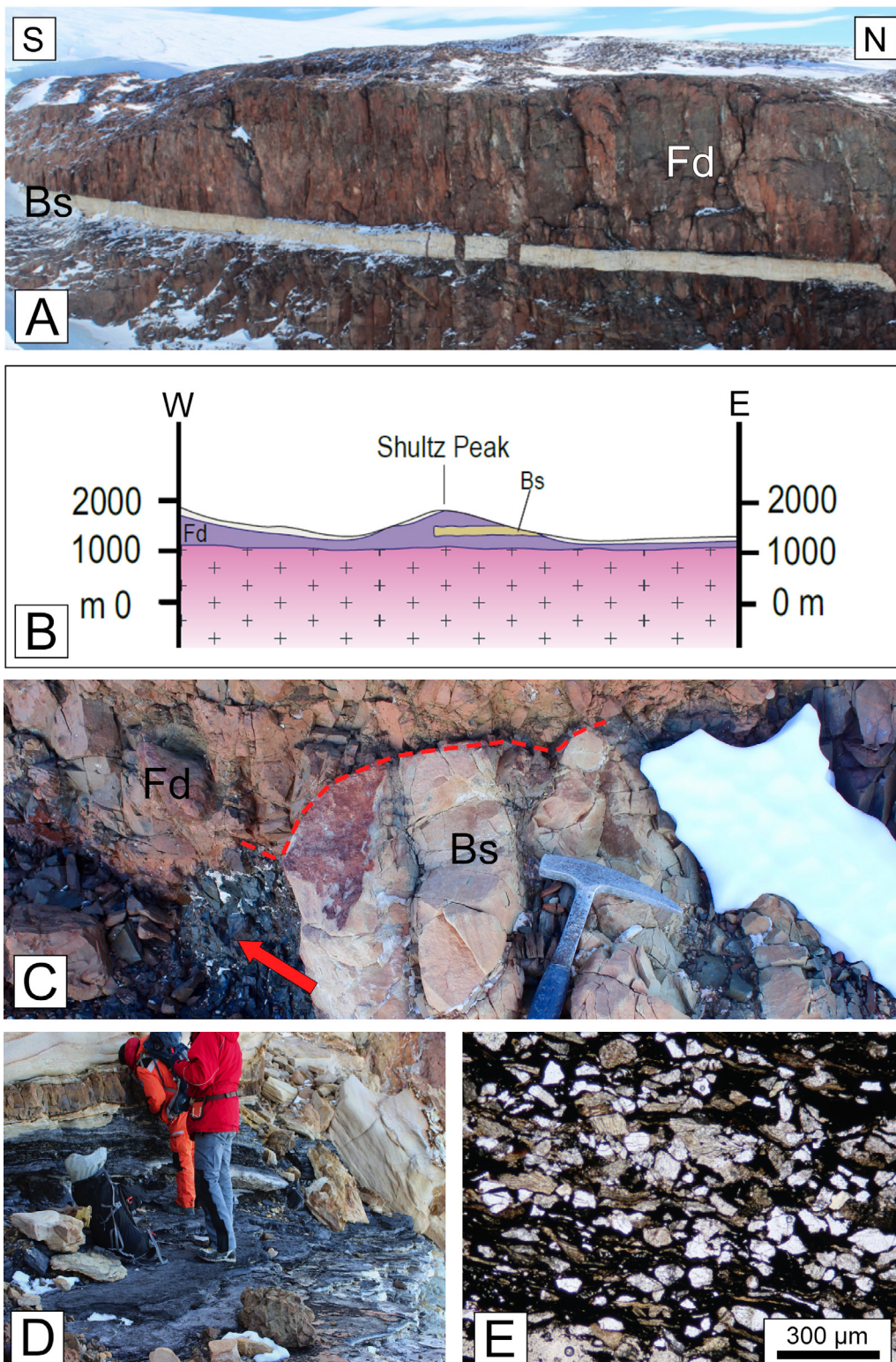
Fig. 5-A) Undifferentiated Beacon sandstone body (Bs), floating in the Ferrar Dolerite (Fd) in the Shultz Peak area. Note that Beacon strata are truncated by the emplacement of the mafic rocks; B) cross section across the Shultz Peak, showing the relations between the Beacon raft (Bs), the Ferrar Dolerite (Fd) and the underlying Granite Harbour Granite; C) beds of Beacon sandstone (Bs), truncated by Ferrar Dolerite (Fd), at the Reckling Peak. Red arrow indicates organic matter; D) beds of Beacon sandstone rich in organic matter at McLea Nunatak; E) microscopic aspect of organic rich levels of Beacon sandstone (parallel Nicols).
