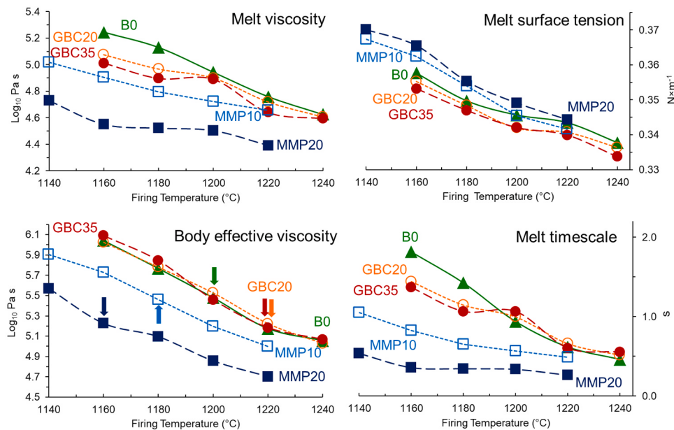
Fig. 8. Trends of calculated shear viscosity ( \text{Log}_{10} \text{ Pa}\cdot\text{s} ), surface tension ( \text{N}\cdot\text{m}^{-1} ) and timescale ( \text{s} ) of the melt, and effective viscosity of the bulk ( \text{Log}_{10} \text{ Pa}\cdot\text{s} ) as a function of firing temperature ( ^{\circ}\text{C} ). Arrows indicate the temperature of maximum densification for each batch. Experimental error is within the symbol size.
