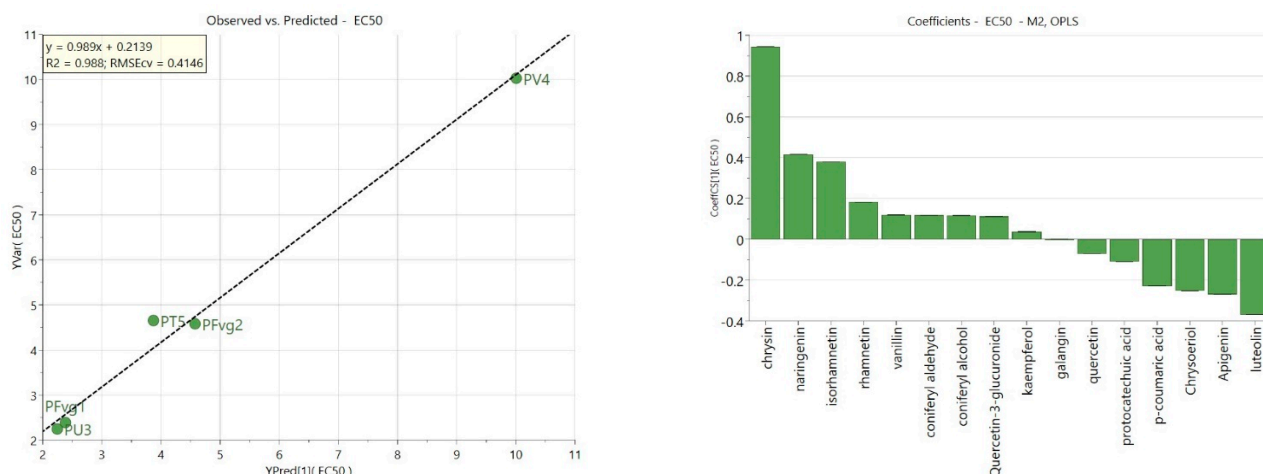
Figure 6. OPLS (Orthogonal Projections to Latent Structures) model analysing propolis extracts to predict their bioactivity, represented by the EC 50 values. ( Left Plot ): relationship between observed and predicted EC 50 values for each propolis sample. ( Right Plot ): coefficients of the model.
