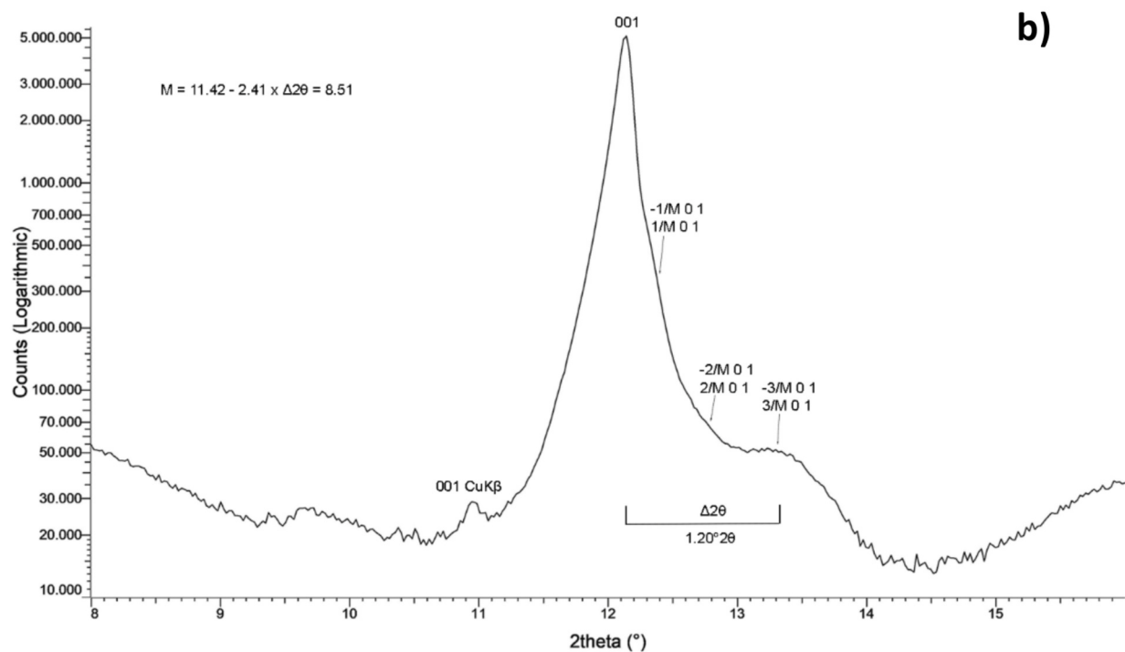
Fig. 5. a) Comparison of the diffraction patterns of pristine antigorite from San Mango (SM Atg) and sample after 1 week of incubation in MGS (SM Atg – 1w); b) magnified view of the diffraction pattern of antigorite from San Mango (intensity shown in logarithmic scale). Position of the first to third-order superstructure reflections is indicated.
