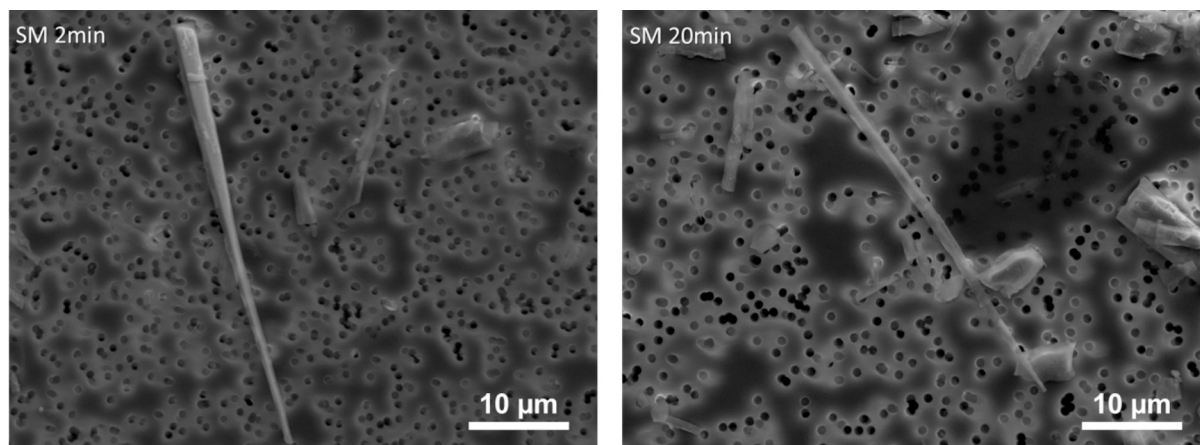
Fig. 4. Representative SEM images of respirable WHO antigorite fibres from San Mango after milling for 2 min and 20 min, showing the asbestos-like morphology.
