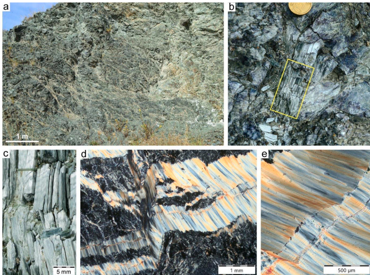
Fig. 2. a) Serpentinite antigorite outcrop of San Mango d'Aquino, showing lens-shaped, dm- to m- large lithons separated by anastomosing cataclastic bands. b) Portion of a cm-large antigorite vein preserved at the margin of an antigorite serpentinite lithon; from this vein portion was sampled the fibrous antigorite studied in this paper. c) Detail of the vein in b); note the mm-large, cm-long lath-shaped fragments derived from the splitting of the vein exposed to weathering agents. d, e) Thin section photomicrographs (cross-polarized light) of cross-fibre, mm-thick Atg veins cut parallel to the fibre elongation. Note the “fibrous” texture of antigorite, particularly evident in e).
