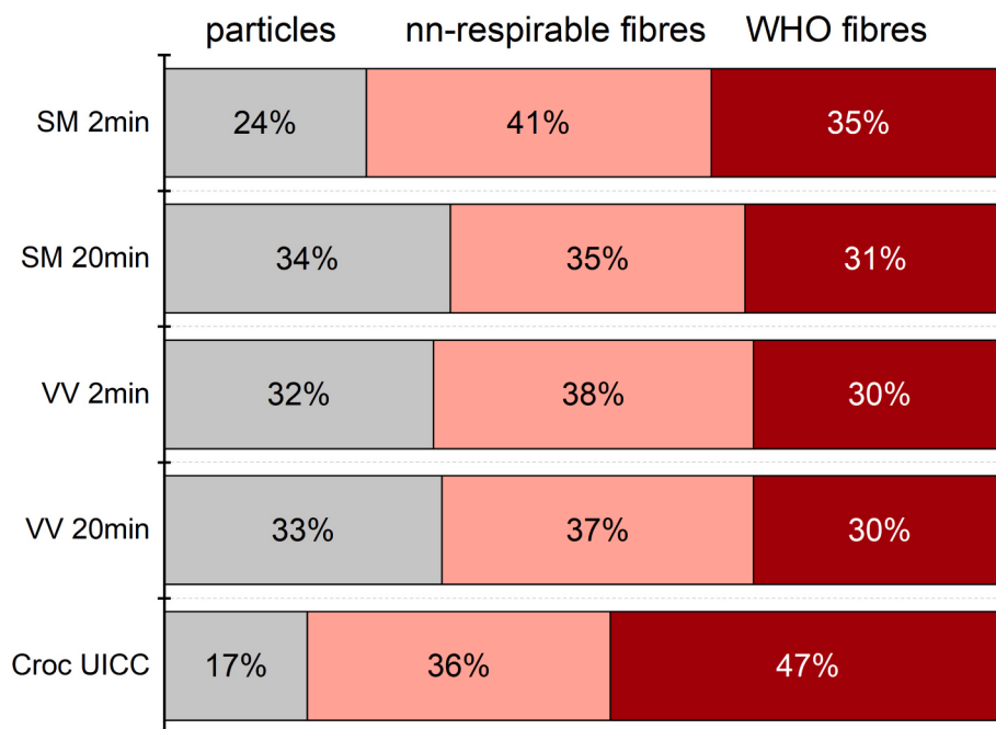
Fig. 3. Particle and fibre distribution of antigorite from San Mango (SM) after standardized mechanical milling (2 and 20 min) detected by optical microscopy and automated image analysis (FPIA). Stacked bar plot shows the % of objects with AR < 3 (particles, grey); AR > 3 (EMPs, according to NIOSH definition [NIOSH, 2011], light red) and respirable WHO fibres (AR > 3, W < 3 \mu m, L > 5 \mu m; [WHO, 1997], red). Varena Valley antigorite (VV; Petriglieri et al., 2023) and UICC crocidolite (Croc UICC) were added for comparison. Full details of particle size distribution of antigorite from San Mango are reported in Supplementary materials S1.
