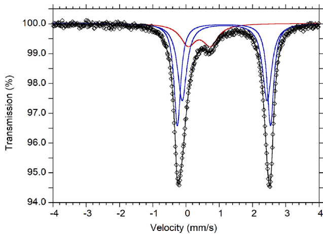
Fig. 7. Room temperature ^{57}\text{Fe} Mössbauer spectrum and parameters of fibrous antigorite from San Mango. Fitted absorption doublets assigned to Fe (II) are indicated in blue and Fe (III) in red. Diamonds denote the measured spectrum, and black curve represents the summed fitted spectrum. The table below the figure shows the ^{57}\text{Fe} Mössbauer parameters for the three doublets: Isomer shift (IS) quadrupole splitting (QS), peak FWHM, and peak area (%).
