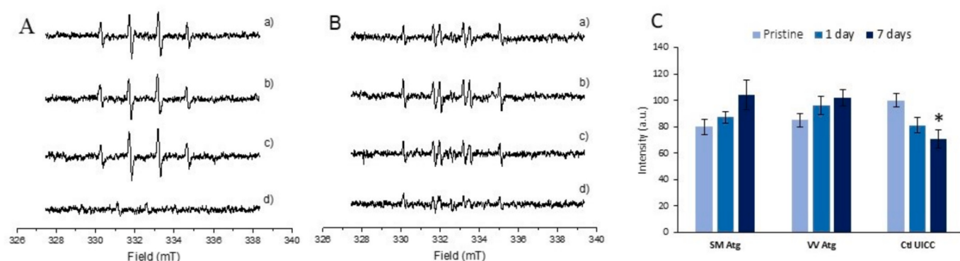
Fig. 9. Representative EPR spectra of (A) [DMPO-OH]• and (B) [DMPO-COO]• adducts recorded for (a) SM Atg, (b) VV Atg, (c) UICC chrysotile, and (d) blank after 1 h of incubation with the target molecule ( \text{H}_2\text{O}_2 for •OH and \text{HCOO}^- for carboxyl radical detection). The [DMPO-OH]• adduct signal is characterized by four peaks with intensity 1:2:2:1 and the [DMPO-COO]• signal by six peaks of equal intensity. The EPR signal of the ascorbyl radical, as intermediate in the oxidation of ascorbic acid to dehydroascorbic acid, was detected (signal at ca. 333 mT in panel B). (C) Amount of •OH radicals generated by the pristine and MGS-incubated (after 1 and 7 days) samples, obtained by double integration of the EPR spectra. Asterisk indicates significant difference between pristine and incubated fibres: * p < 0.05 (one-way ANOVA followed by post-hoc Tukey's test). Data for VV Atg and UICC chrysotile fibres from Petriglieri et al. (2023) are reported for comparison.
