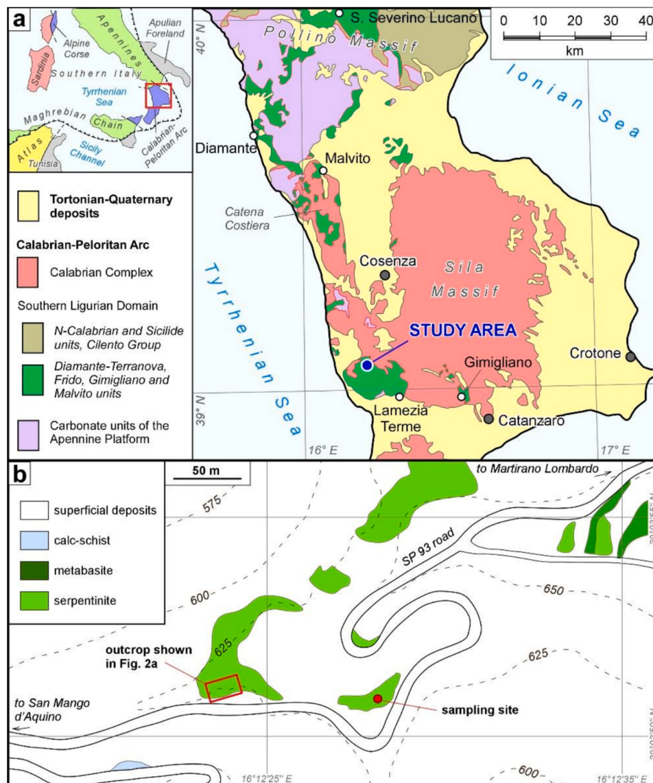
Fig. 1. a) Geological scheme of northern Calabria showing the distribution of the ophiolite-bearing units of the Southern Ligurian Domain and the position of the study area; modified after Amodio-Morelli et al. (1976) . The inset shows the position of northern Calabria (red rectangle) in southern Italy. b) Scheme of the sampling area showing the position of the ophiolite outcrops and of the sampling site.
