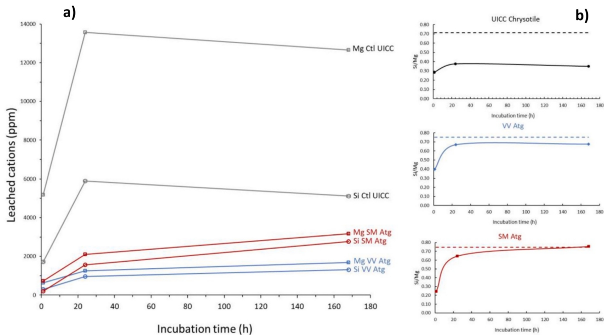
Fig. 8. a) Si and Mg release as a function of the incubation time of fibrous antigorite from San Mango (SM Atg). Results on antigorite from Val Varenna (VV Atg) and UICC chrysotile (Ctl UICC) are reported for comparison. Values are reported as means \pm SD; b) variation of Si/Mg ratio in solution as a function of sample incubation time. Bulk Si/Mg ratio (dotted line) obtained from chemical analyses (by EMP) of the pristine sample is reported for comparison.
