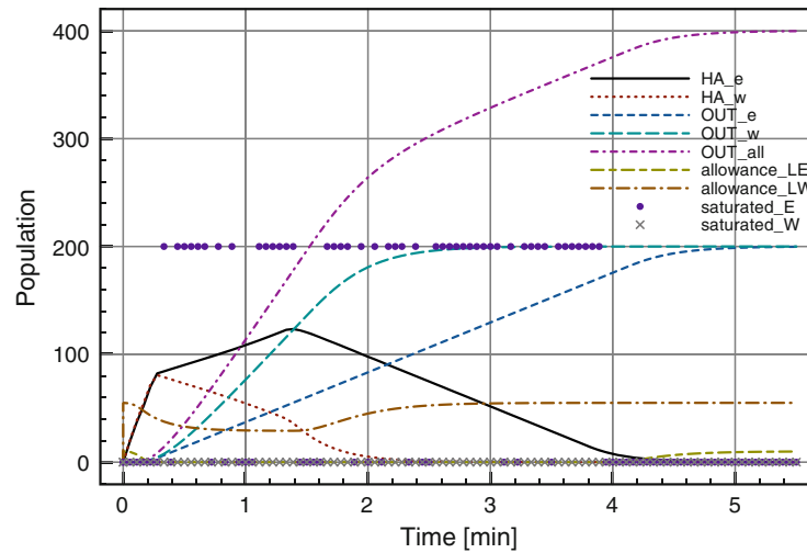
Fig. 16. Bio-PEPA Emergency Egress: Rerouting (ODE)
