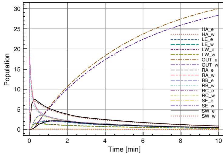
Fig. 12. Bio-PEPA Emergency Egress: No Routing
