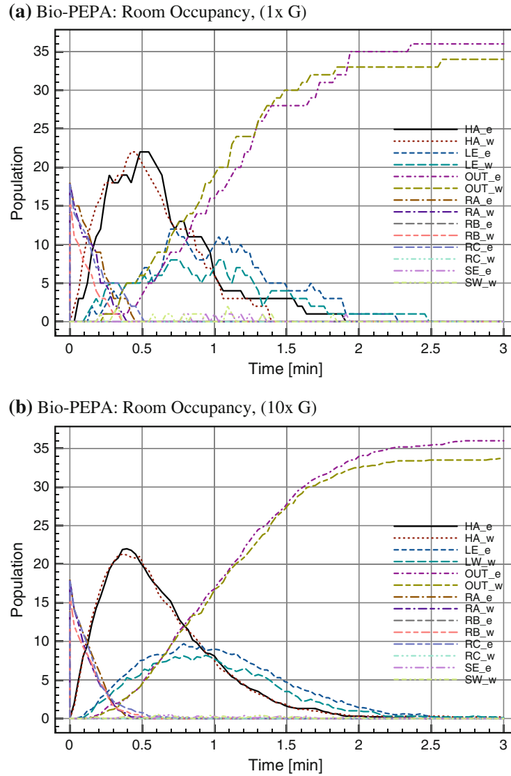
Fig. 10. Bio-PEPA Emergency Egress: ( 1 \times G ) and ( 10 \times G ) Simulation Results.
