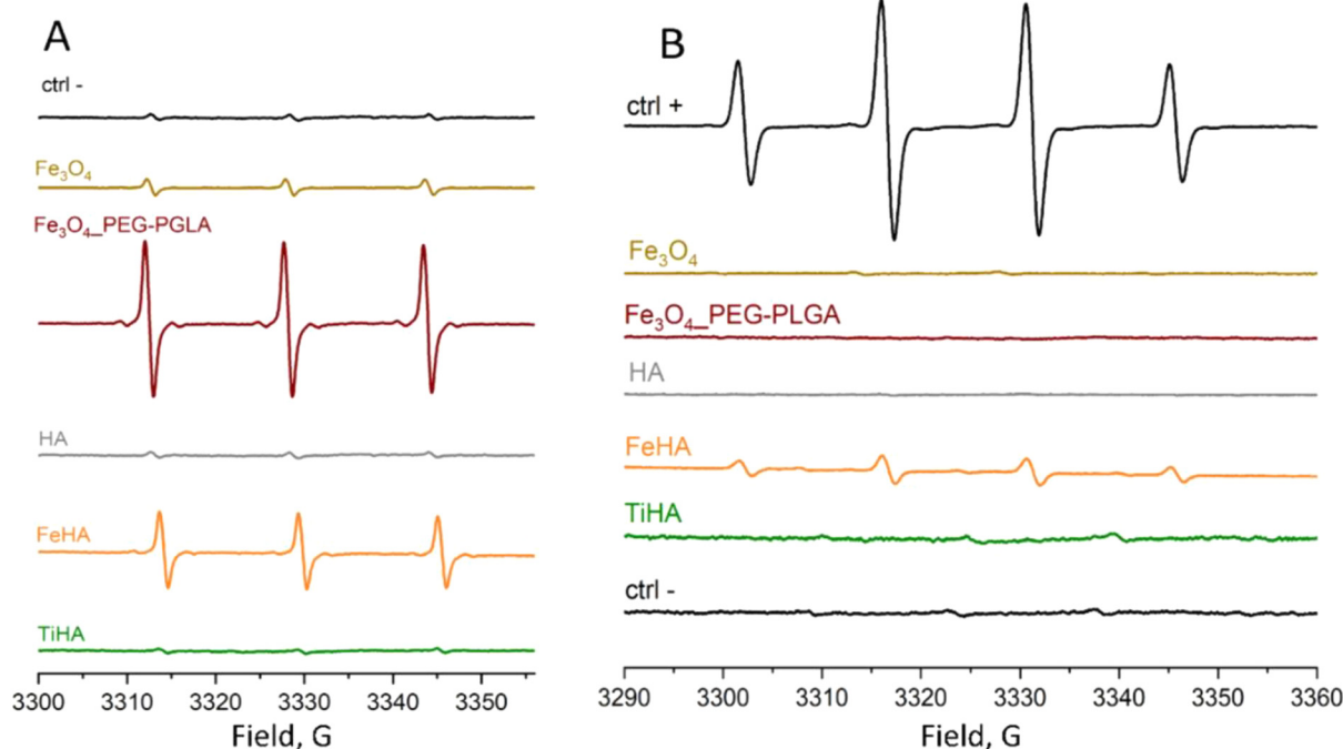
Fig. 4 EPR spectra. (A) Surface reactivity assessed using the TEMPONE-H probe molecule as a spin trap; (B) Fenton-like reactivity with the addition of hydrogen peroxide assessed using DMPO as a spin trap. Conditions: NBMs in phosphate buffer at pH 7.4.
