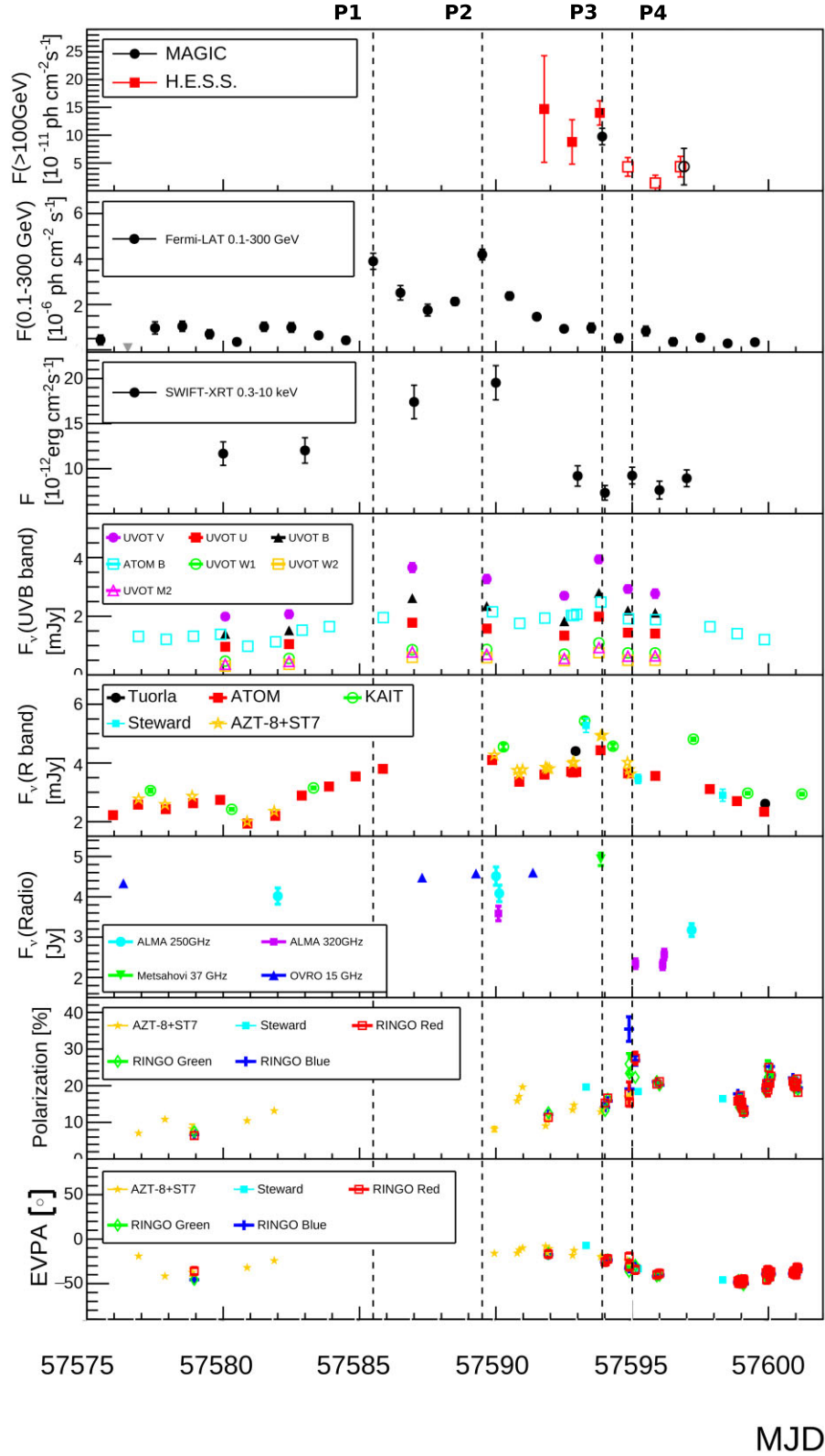
Figure 2. MWL light curves of OT 081 during the period from MJD 57575 to MJD 57602 (2016 July 6–August 2). Vertical dashed lines P1 (MJD 57585.5 – 2016 July 16), P2 (MJD 57589.5 – 2016 July 20), P3 (MJD 57593.9 – 2016 July 24), and P4 (MJD 57595 – 2016 July 26) indicate the four states of the source, which were identified. The empty circle and empty squares in the top panel correspond to flux points derived for the low-significance data set, compatible with the background-only hypothesis. In the panel corresponding to Fermi -LAT light curve (second panel from the top), the downward-facing triangle corresponds to a UL.
