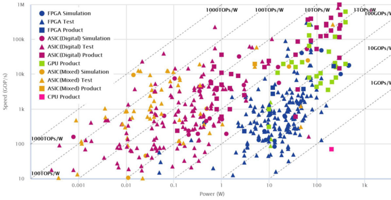
Fig. 2. Overview on state-of-the-art Neural Network accelerators based on available data collected in [76]. Legenda: Simulation means GOPS/W values collected from post-layout simulation; Test means from prototype devices; Product means from off-the-shelf devices.
