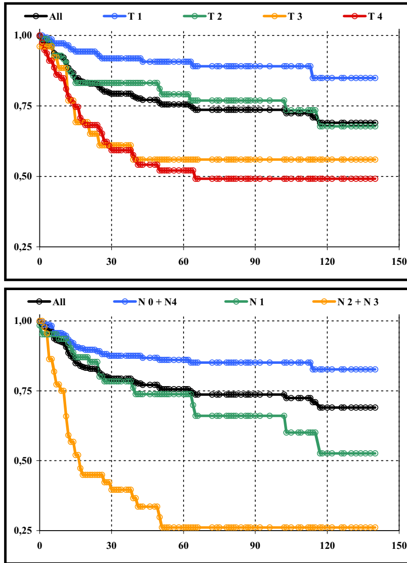
FIGURE 2. Survival curves according to size and node involvement of OSCC.
