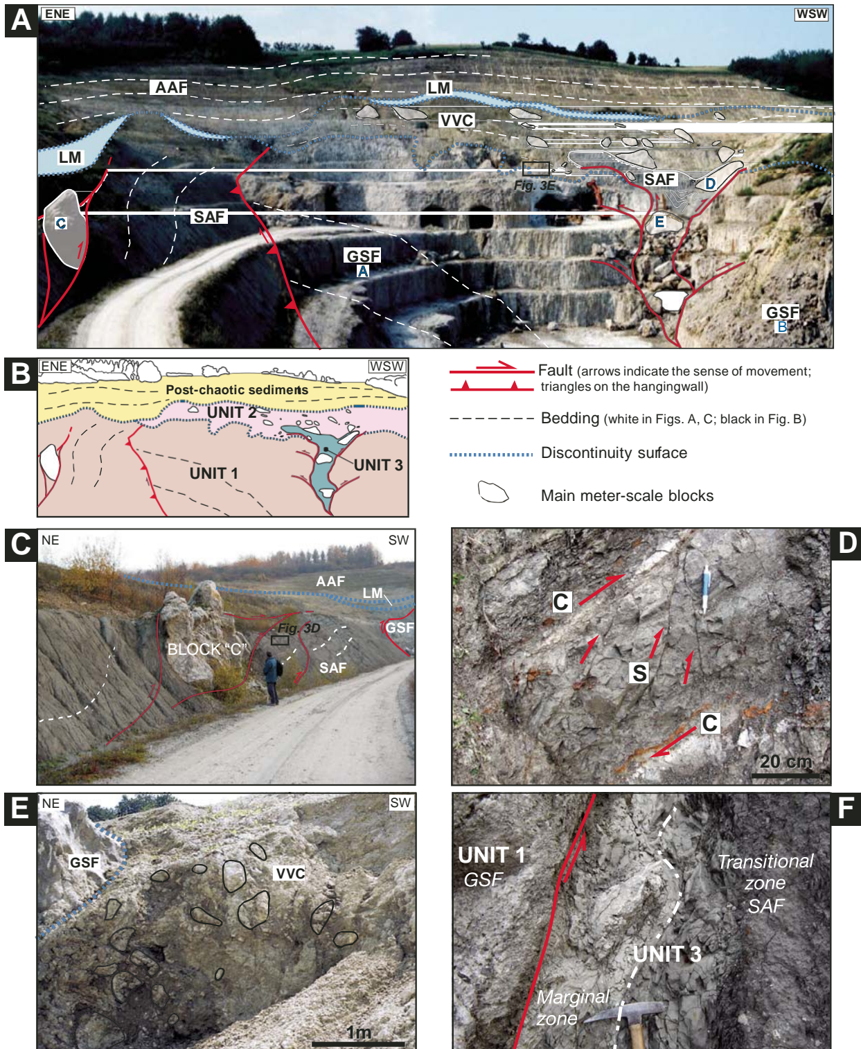
Figure 3. (A) Panoramic view of the Moncucco quarry. SAF—Sant’Agata Fossili marls (upper Tortonian-lower Messinian); GSF—Gesso Solifera Formation (Messinian); VVC—Valle Versa chaotic complex (upper Messinian); LM—Lago-Mare deposits (upper Messinian); AAF—Argille Azzurre Formation (lower Pliocene). Capital letters (A–E) indicate the blocks described in the text. (B) Drawing of Figure 3A, showing the distribution of the three chaotic units discussed in the text. (C) Unit 1: lozenge-shaped gypsum block tectonically included within the SAF (block C, Fig. 3A). Symbols as in A. (D) Unit 1: S-C structures in the SAF marls. The C planes coincide with the bedding surfaces. Red arrows indicate the sense of shear. Location in C. (E) Unit 2: VVC: angular to rounded gypsum and carbonate blocks floating in a fine-grained matrix. See A for location. (F) Tectonic contact separating Unit 1 and Unit 3. The boundary between the marginal and the transitional zones is also shown (white dotted line). See Figure 7A for location.
