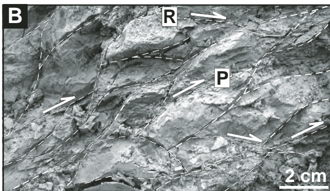
Figure 5. Unit 1. (A) Cyclic organization of the Gessoso Solifera Formation (GSF, block “A”), evidenced by the alternation of decimeter-thick mudstone beds (white dashed lines) and thick selenitic gypsum beds, their base outlined by white V-shaped symbols (top to the right). The transpressive faults juxtaposing the gypsum blocks “A” and “C” to the Sant’Agata Fossili marls (SAF) can be seen. Black dotted lines indicate the bedding of SAF. Diggers on the right give scale. (B) Centimeter-spaced L shear lenses defined by the interlacing of R and P shears (white dashed lines) in the Sant’Agata Fossili marls. Arrows indicate the sense of shear. See A for location.
