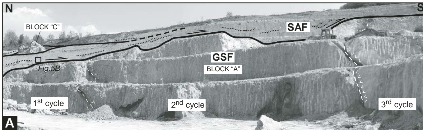
Figure 5. Unit 1. (A) Cyclic organization of the Gessoso Solifera Formation (GSF, block “A”), evidenced by the alternation of decimeter-thick mudstone beds (white dashed lines) and thick selenitic gypsum beds, their base outlined by white V-shaped symbols (top to the right). The transpressive faults juxtaposing the gypsum blocks “A” and “C” to the Sant’Agata Fossili marls (SAF) can be seen. Black dotted lines indicate the bedding of SAF. Diggers on the right give scale. (B) Centimeter-spaced L shear lenses defined by the interlacing of R and P shears (white dashed lines) in the Sant’Agata Fossili marls. Arrows indicate the sense of shear. See A for location.
