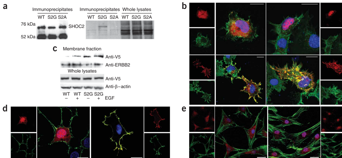
Figure 2 The disease-causing 4A>G change in SHOC2 promotes protein myristoylation and cell membrane targeting. (a) [ ^3\text{H} ]Myristic acid incorporation (middle) occurs in SHOC2 S2G but not in SHOC2 wt or SHOC2 S2A . Equivalent levels of SHOC2 proteins in immunoprecipitates (left) and [ ^3\text{H} ]myristic acid incorporation in cells (right) are shown. (b) SHOC2 wt is uniformly present in the cytoplasm and nucleus in starved Cos-1 cells (upper left) and is restricted to the nucleus following EGF stimulation (upper right), whereas SHOC2 S2G is targeted to the cell membrane basally (lower left) and after stimulation (lower right). Confocal microscopy visualized SHOC2 (anti-V5 monoclonal, then Alexa Fluor 594–goat anti-mouse; red), actin cytoskeleton (Alexa Fluor 488–phalloidin; green) and nuclei (DAPI; blue). (c) Cell fractionation assay documenting preferential membrane targeting of SHOC2 S2G . The protein ERBB2 is shown to demonstrate equivalent fractionation efficiency, whereas anti-V5 blots from cell lysates show equivalent transfection efficiency. (d) Colocalization of V5-tagged SHOC2 S2G and ganglioside M1 to the plasma membrane in Cos-1 cells. Subcellular localization of V5-tagged wild-type SHOC2 (left) and V5-tagged SHOC2 S2G (right) is shown. Ganglioside M1 was detected by using the Vybrant Lipid Raft Labeling kit (green). SHOC2 proteins and nuclei are visualized as reported above. (e) Subcellular localization of the endogenous SHOC2 wt protein in primary skin fibroblasts, basally (left) and after stimulation (right). Confocal microscopy was performed using an anti- SHOC2 polyclonal followed by Alexa Fluor 594–goat anti-rabbit (red), whereas the actin cytoskeleton was detected by Alexa Fluor 488–phalloidin (green). All images are single optical sections representative of > 50 transfected cells observed in each experiment. Bars, 20 \mu\text{m} ( b,d ) or 40 \mu\text{m} ( e ).
