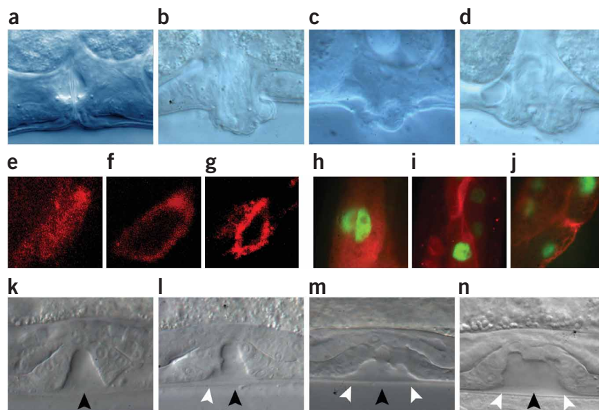
Figure 4 Consequences of SHOC2 S2G expression in C. elegans vulva development. (a–d) Nomarski images of vulvas of adult animals. A normal vulva is observed in animals expressing SHOC2 wt (a) , whereas in worms expressing SHOC2 S2G (b,c) or myr::SHOC2 wt (d) a protrusion of the vulva is visible. (e–j) Subcellular localization of V5-tagged SHOC2 proteins in C. elegans cells. In excretory canal cells (e–g) and intestinal cells (h–j) , SHOC2 wt protein is present throughout the cytoplasm (e,h) , whereas both SHOC2 S2G (f,i) and myr::SHOC2 wt (g,j) are enriched in or restricted to the plasma membrane. Anti-V5 (red) was used to visualize SHOC2 proteins. In intestinal cells, nuclei express GFP due to pelt-2::GFP plasmid used as a marker for transformation. (k–n) Nomarski images of vulval precursor cells at the L3 stage. In animals expressing SHOC2 wt only P6.p descendants invaginate (k) , whereas in SHOC2 S2G - (l,m) and myr::SHOC2 wt -expressing (n) animals, P5.p (l–n) and P7.p descendants (m,n) also detach from the cuticle. Black arrowheads point to P6.p descendant invagination, whereas white arrowheads point to P5.p and P7.p descendant invagination. Anterior is to the left and dorsal is up in all images.
