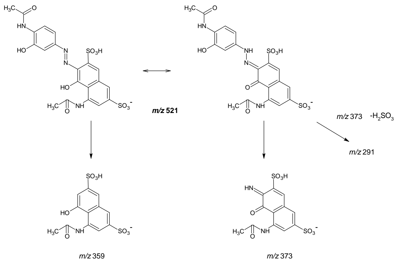
Scheme 4. Key fragmentation pathways followed by AV7.
