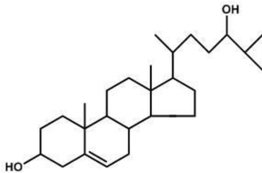
24-HYDROXY-CHOLESTEROL (24-OH)
