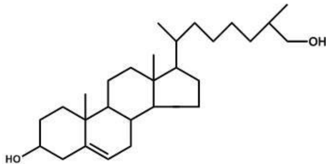
27-HYDROXY-CHOLESTEROL (27-OH)
