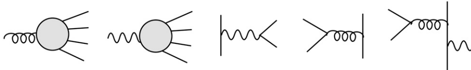
Fig. 6. Gluon exchange subdiagrams.
