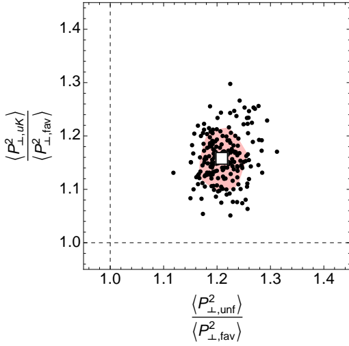
Figure 2. Kinematic-independent distribution of average squared transverse momenta in TMD FFs: \langle P^2_{\perp,unf} \rangle / \langle P^2_{\perp,fav} \rangle vs. \langle P^2_{\perp,uK} \rangle / \langle P^2_{\perp,fav} \rangle .
