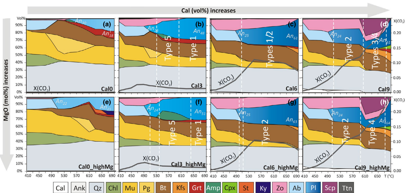
FIGURE 8 Modebox plots of changes in calculated mineral proportions and fluid composition ( X(\text{CO}_2) , dotted black lines) during prograde metamorphism along the internal buffered P/T - X(\text{CO}_2) paths reported in Figure 6: (a, e) Cal0, (b, f) Cal3, (c, g) Cal6, (d, h) Cal9 model bulk compositions with variable MgO concentrations. Plagioclase is reported in blue, with progressively darker tones for increasing anorthite contents (mainly from oligoclase to labradorite compositions, as reported in each diagram). Types 1–5 refer to the main lithologies recognized in the studied calcic metapelites from the LHS and GHS of Nepal Himalaya (see Figures 1 and 2) [Colour figure can be viewed at wileyonlinelibrary.com ]
