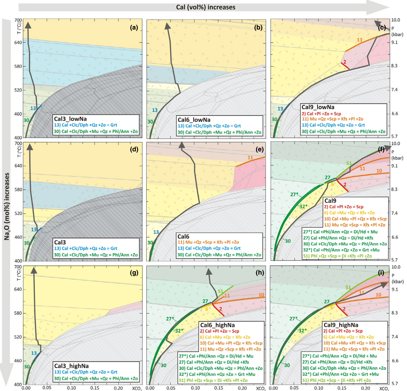
FIGURE 11 Results of phase equilibria modelling for Cal3 (a, d, g), Cal6 (b, e, h) and Cal9 (c, f, i) model bulk compositions with variable \text{Na}_2\text{O} concentrations (same P/T-X(\text{CO}_2) pseudosections as in Figure 7) showing the main decarbonation reactions relevant for calcic metapelites (reactions labels and colours as in Figure 5). The dashed arrows are the same P/T-X(\text{CO}_2) paths as in Figure 7 (i.e. fluid-rock buffering paths according to a constant porosity model) [Colour figure can be viewed at wileyonlinelibrary.com ]
