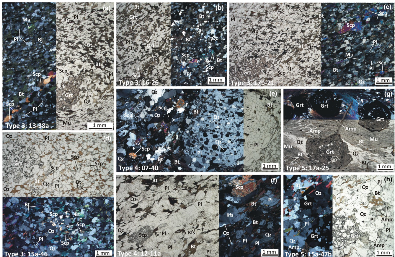
FIGURE 2 Representative microstructures and mineral assemblages of Type 3 (a–d), type 4 (e, f) and Type 5 (g, h) calcic metapelites from LHS and GHS of Nepal Himalaya. (a) Garnet+scapolite-bearing two-micas schist: note that biotite is significantly more abundant than muscovite. Scapolite is mostly concentrated in lens-like domains (PPL, XPL). (b) Garnet+scapolite-bearing biotitic schist: garnet porphyroblasts have a skeletal habit and scapolite is concentrated in millimetric lenses (PPL, XPL). (c) Garnet+scapolite-bearing two-micas schist, with biotite less abundant than muscovite. Scapolite is mostly concentrated in lens-like domains (PPL, XPL). (d) Garnet+scapolite-bearing biotitic gneiss: note the skeletal habit of garnet and the fine-grained scapolite dispersed in the matrix (PPL, XPL). (e) Plagioclase+scapolite-bearing biotitic gneiss: plagioclase occurs in pluri-mm poikiloblasts including quartz, whereas scapolite is associated with the biotite layers (PPL, XPL). (f) Scapolite+plagioclase biotitic gneiss: both plagioclase and scapolite are granoblastic (PPL, XPL). (g) Two-micas, garnet+amphibole-bearing phylladic micaschist: garnet porphyroblasts include an internal rotated foliation, whereas the colourless amphibole porphyroblasts statically overgrow the main foliation (PPL, XPL). (h) Garnet+amphibole-bearing biotitic gneiss: garnet has a skeletal habit and amphibole is pale-green (PPL, XPL) [Colour figure can be viewed at wileyonlinelibrary.com ]
