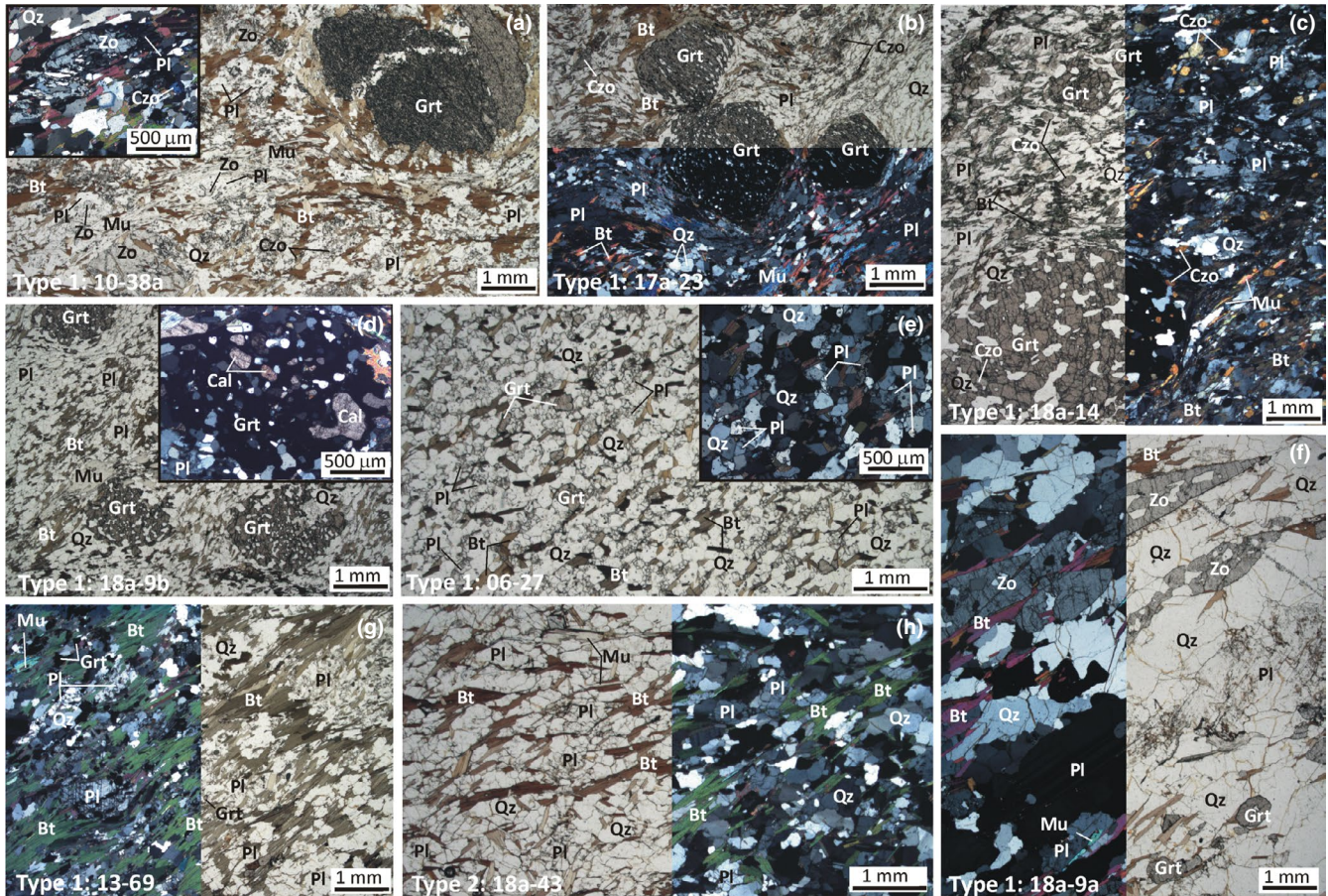
FIGURE 1 Representative microstructures and mineral assemblages of Type 1 (a–g) and Type 2 (h) calcic metapelites from the Lesser Himalayan Sequence (LHS) and Greater Himalayan Sequence (GHS) of Nepal Himalaya. (a) Garnet+zoisite plagioclase-bearing two micas-schist. Garnet and zoisite occur as pluri-mm porphyroblasts, whereas plagioclase is dispersed in the matrix and replaces zoisite (Plane Polarized Light, PPL). The inset shows a detail of zoisite partially replaced by plagioclase (Crossed Polarized Light, XPL). (b) Garnet+plagioclase two micas-schist; garnet and plagioclase are, respectively, porphyroblasts syn- and post-kinematic with respect to the main foliation (PPL, XPL). (c) Garnet+plagioclase+clinozoisite biotitic schist: garnet poikiloblasts include quartz, plagioclase and clinozoisite (PPL, XPL). (d) Garnet+plagioclase-bearing biotitic gneissic micaschist: garnet porphyroblasts are syn-kinematic with respect to the main foliation, whereas plagioclase overgrows it (PPL). The inset shows a detail of a garnet porphyroblast with relict calcite inclusions (XPL). (e) Plagioclase+garnet-bearing biotitic gneiss: note the high relief of plagioclase, which is interstitial between quartz and biotite (PPL; inset, XPL). (f) Zoisite+plagioclase+garnet-bearing biotitic gneiss: zoisite and plagioclase are coarse-grained and mostly aligned to the main foliation (PPL, XPL). (g) Plagioclase+garnet-bearing biotitic schist: plagioclase statically overgrows the main foliation defined by biotite (PPL, XPL). (h) Plagioclase-bearing biotitic gneissic micaschist: note the high relief of plagioclase, which is dispersed in the matrix (PPL, XPL)
