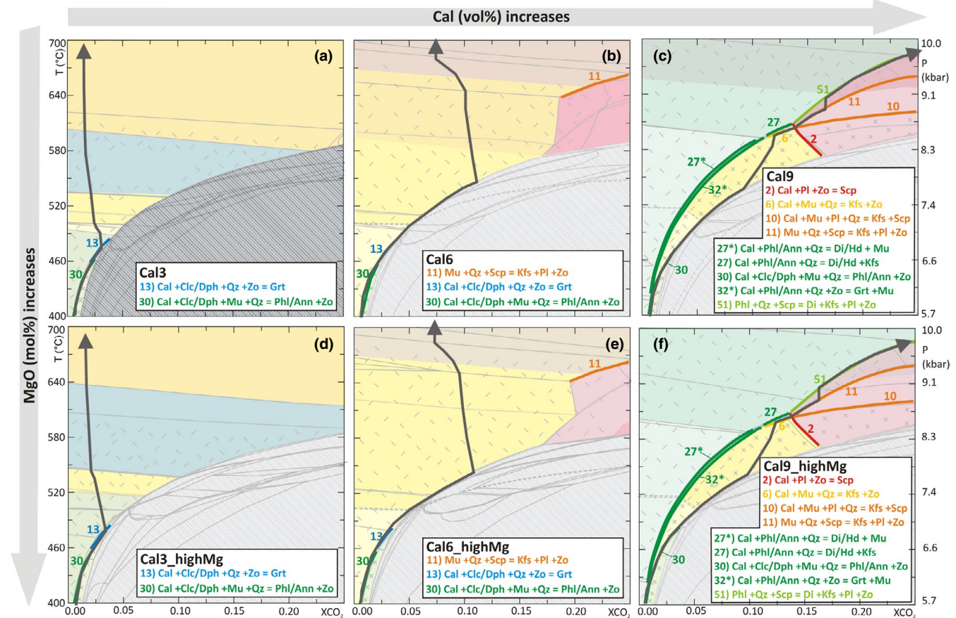
FIGURE 10 Results of phase equilibria modelling calculation for Cal3 (a, d), Cal6 (b, e) and Cal9 (c, f) model bulk compositions with variable MgO concentrations (same P/T-X(\text{CO}_2) pseudosections as in Figure 6) showing the main decarbonation reactions relevant for calcic metapelites (reactions labels and colours as in Figure 5). Note that the univariant curves overlap the (narrow) di- and tri-variant fields of the underlying pseudosections. The dashed arrows are the same P/T-X(\text{CO}_2) paths as in Figure 6 (i.e. fluid-rock buffering paths according to a constant porosity model) [Colour figure can be viewed at wileyonlinelibrary.com ]
