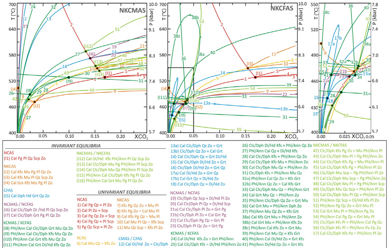
FIGURE 5 P/T-X(\text{CO}_2) projections calculated along a P/T gradient typical of collisional orogenic settings, showing invariant and univariant equilibria for the NKCMAS– \text{H}_2\text{O}-\text{CO}_2 and NKCFAS– \text{H}_2\text{O}-\text{CO}_2 sub-systems. The large black circles are invariant points; the small, white circles are singular points [Colour figure can be viewed at wileyonlinelibrary.com ]
