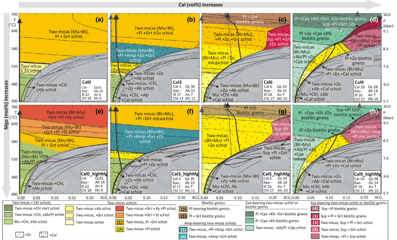
FIGURE 6 Results of phase equilibria modelling calculation for Cal0 (a, e), Cal3 (b, f), Cal6 (c, g) and Cal9 (d, h) model bulk compositions with variable MgO concentrations: (a–d) ‘average’-MgO compositions; (e–h) MgO-enriched compositions. Rock types are defined according to the main mineral assemblages; phase abundances lower than 1 vol.% are considered irrelevant for the definition of the main lithologies. Distinction among schists and gneisses is based on the modal amount of phyllosilicates (i.e. >25 vol.% for schists, <25 vol.% for gneisses). Numbers from 1 to 5 in the legend refer to the main lithological types recognized in the studied calcic metapelites from the LHS and GHS of Nepal Himalaya (see Figures 1 and 2). The insets in each diagram refer to the approximate protolith’s mineral composition as reported in Figure 4. The grey arrows are the hypothetical, yet quantitative, P/T-X(\text{CO}_2) paths followed by each model composition in the hypothesis that the system remained internal buffered along the whole prograde evolution: continuous line = fluid-rock buffering path according to a constant porosity model (i.e. the fluid is allowed to accumulate within the rock until it reaches a specified threshold, after which fluid loss occurs); dotted line = fluid-rock buffering path in a completely closed system (i.e. no fluid loss is allowed); dashed line = fluid-rock buffering path in a completely open system (i.e. all the fluid that is produced is immediately lost). The grey dashed field in each diagram is the stability field of ankerite–dolomite and is not considered in this study. Details on field assemblages, mineral abundances and plagioclase composition are given in Figures S2–S4 [Colour figure can be viewed at wileyonlinelibrary.com ]
