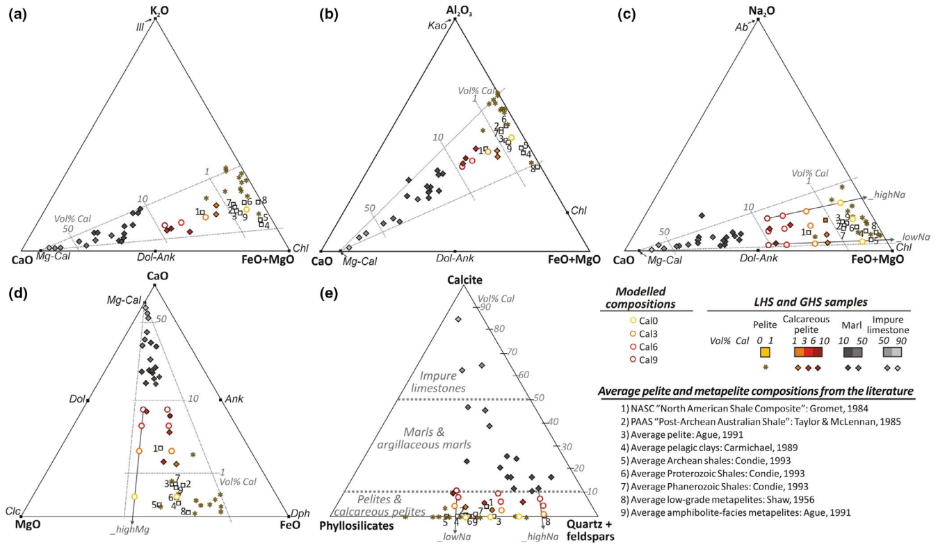
FIGURE 3 Measured and model bulk-rock compositions for a wide range of meta-sediments discussed in this paper, plotted in the CaO–K 2 O–(FeO+MgO) (a), CaO–Al 2 O 3 –(FeO+MgO) (b), CaO–Na 2 O–(FeO+MgO) (c), CaO–MgO–FeO (d) compositional diagrams (mol.%), as well as in the phyllosilicate–calcite–(quartz+feldspars) ternary diagram (e) (vol.%). The coloured diamonds refer to Himalayan meta-sediments derived from calcareous pelites (orange to dark red), marls (dark grey) and impure limestones (light grey); the yellow asterisks refer to Himalayan meta-sediments derived from pelites sensu stricto. The numbered squares are average pelite or metapelite compositions from the literature (see the legend), whereas the circles with a coloured contour represent the model bulk compositions used for thermodynamic modelling. Vol.% of calcite reported in (a), (b), (c) and (d) (grey dotted lines) refer to the reconstructed approximate protolith's mineral compositions (see text for further explanation) and are coherent with those reported in (e) and in Figure 4 [Colour figure can be viewed at wileyonlinelibrary.com ]
