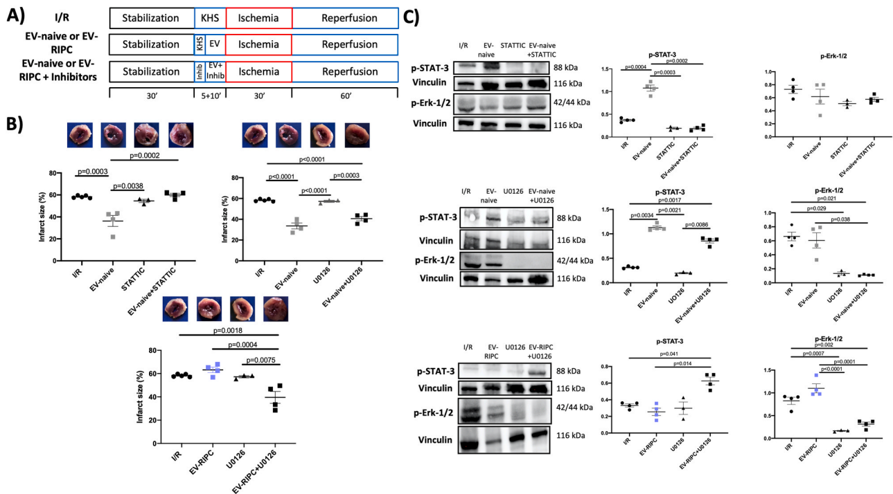
Fig. 4. EV-naive protection relies on STAT-3 phosphorylation. (A) Timeline of ex-vivo I/R protocol. The hearts were infused with either STATTIC or U0126 alone ( n = 3 /each inhibitor) for 5 min followed by EV-naive or EV-RIPC for 10 min ( n = 4 /each group). (B) Infarct size in isolated rat hearts treated with EV-naive or EV-RIPC with or without STATTIC or U0126. (C) Western blot analysis and histograms of myocardial tissues recovered upon EV-naive and EV-RIPC untreated or pre-treated with STATTIC or U0126. p-STAT-3 and p-Erk-1/2 expression were normalized to vinculin.
