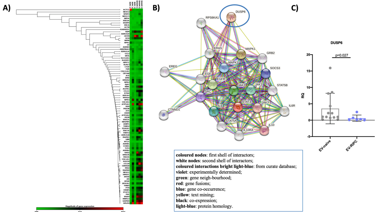
Fig. 5. Heatmap, network platform and DUSP6 validation. (A) Hierarchical clustering of the entire dataset of expressed cardiovascular-linked genes. Clustergram displaying hierarchical clustering of the entire dataset of expressed genes across two different experimental groups: EV-RIPC and EV-naive ( n = 3 /each group). RNAs with higher differential expression levels are represented in red, while RNAs with lower detection levels are shown in green. Genes with similar expression patterns are grouped. (B) String Database functional association network platform. Filtered and assessed functional genomic data exploring the predicted interaction networks. (C) DUSP6 mRNA expression in EV-naive and EV-RIPC by qRT-PCR ( n = 30 ).
