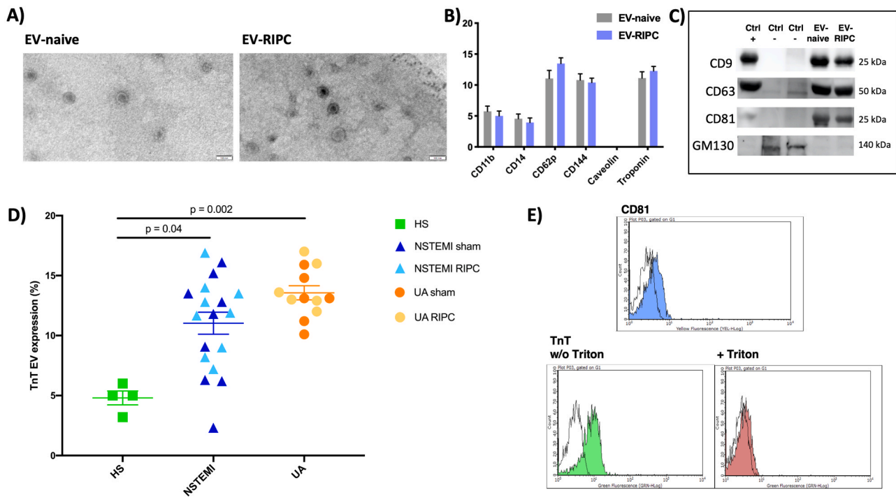
Fig. 2. Characterization of EV-naive and EV-RIPC. (A) Representative images of TEM performed on EV-naive and EV-RIPC (n = 3/each group). Original magnification 140 K, scale bar: 100 nm. (B) EV-naive and EV-RIPC flow cytometry analysis performed with GUAVA FACS. (C) Representative western blot of exosomal markers, CD9, CD63 and CD81, detected in serum-derived EV (Ctrl+), EV-naive and EV-RIPC. GM130 protein served as negative marker of EV (n = 3/each group). (D) EV-TnT expression (%) in all patients and in four healthy subjects. (E) Representative images reporting the exosomal marker CD81 and EV-TnT content before (left panel) and after Triton X100 treatment (right panel) (n = 4). *HS=Healthy subjects.
