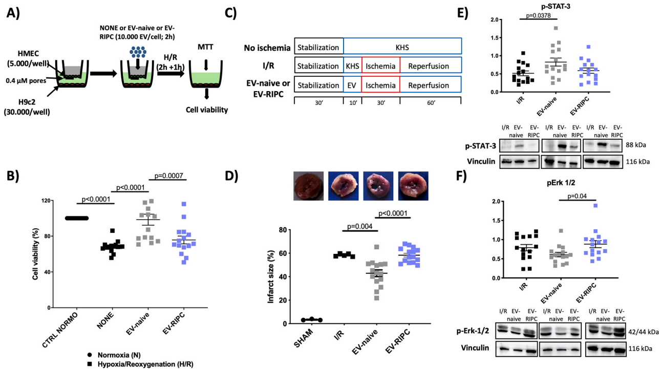
Fig. 3. EV-naive, unlike EV-RIPC, protect H9c2 cells from H/R injury and the heart from IRI. (A) Experimental protocol using the trans-well assay. HMEC-1 were treated with EV-naive or EV-RIPC (2 h), or left untreated, and subjected to the H/R protocol (H2h/R1h). (B) Cell viability on H9c2 cells. The MTT assay was performed on H9c2 cells using EV-naive and EV-RIPC Data were normalized to the mean value of normoxic control (n = 30). (C) Timeline of ex-vivo I/R protocol. The hearts were subjected to 30 min of global ischemia, followed by 60 min of reperfusion. EV was infused for 10 min before ischemia. (D) Infarct size in isolated rat hearts, treated as indicated. The necrotic mass was measured at the end of reperfusion and reported as percentage of the left ventricle mass (LV; % IS/LV). (E-F) Representative Western blot analysis and histograms of myocardial tissues after EV-naive and EV-RIPC treatment. p-STAT-3 and p-Erk-1/2 expression were normalized to vinculin (n = 30).
