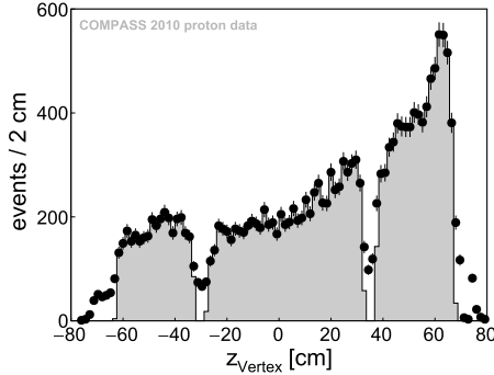
Fig. 2. Distribution of z -coordinate of reconstructed primary vertices. The accepted events are denoted by the shaded area.
