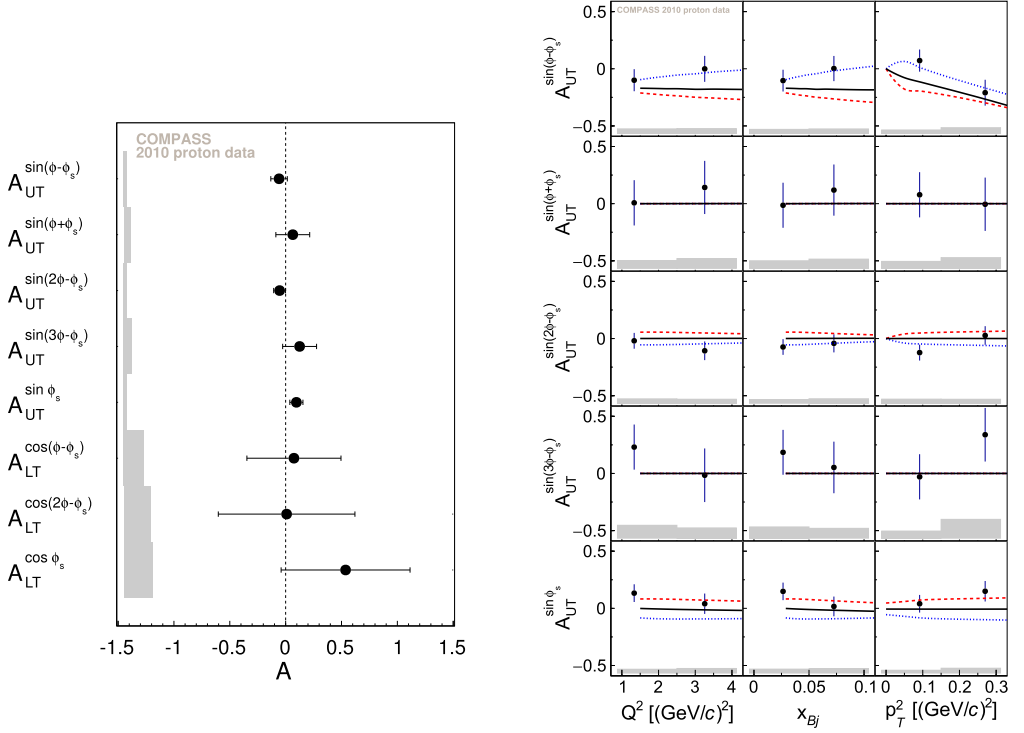
Fig. 8. Left: Average azimuthal asymmetries for exclusive \omega muoproduction. The error bars (left bands) represent the statistical (systematic) uncertainties. Right: Single spin azimuthal asymmetries as a function of Q^2 , x_{Bj} and p_T^2 . The curves show the predictions of the GPD-based model [15] for the average Q^2 , W and p_T^2 values of the COMPASS data. The dashed red and dotted blue curves represent the predictions with the positive and negative \pi\omega form factors, respectively, while the solid black curve represents the predictions without the pion pole.
