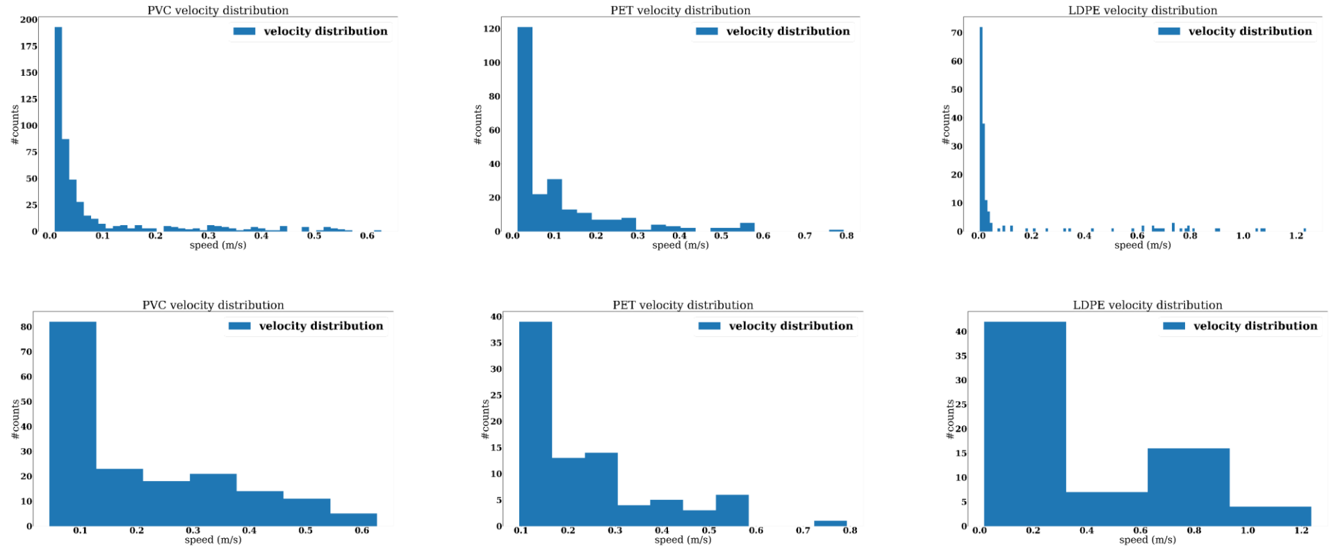
Figure SM1. Histograms of the settling velocity distribution for the n^{\text{th}} = 70^{\text{th}} (top) and the n^{\text{th}} = 90^{\text{th}} (bottom) percentile thresholds for PVC (left), PET (centre) and LDPE (right) fragments.
