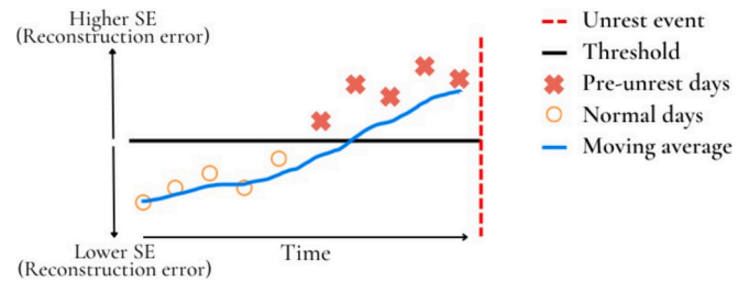
Fig. 3. Reconstruction error plot of the ideal model , where all "normal" days, i.e. days far from the unrest event – are represented by orange circles, and have a lower squared error than the "pre-unrest" days, i.e. the days near the unrest event, represented by coral crosses. A clear separation by threshold is possible: the horizontal black line represents the threshold for separating "normal" days from "pre-unrest" days. A moving average – the blue line – had to be included due to the potential for fluctuations in the squared error for a single day in real-world scenarios. This is achieved by computing the squared error over the most recent 15 days, instead of solely relying on the score of a single day. As a result, the moving average provides a more robust indication of potential unrest when it surpasses the threshold, as it considers a larger squared error sample size. (For interpretation of the references to colour in this figure legend, the reader is referred to the web version of this article.)
